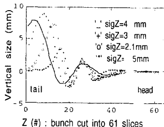
Figure 5. Simulated beam vertical size distortions at the end of the Sector-1
