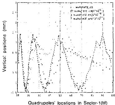
Figure 4. Simulated vertical trajectories in Sector-1.
