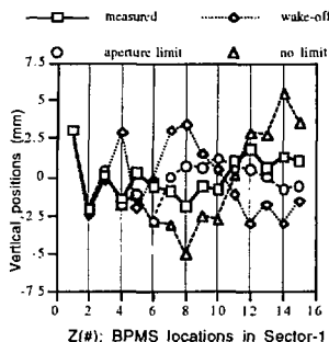
Figure 6. Simulation and measured results of beam trajectory versus BPMs.
