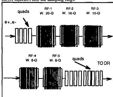
Figure 1. The layout of the SLC injector linac
