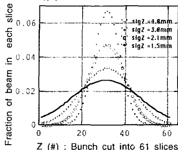
Figure 3. Percentage of number of particles in each slice.
