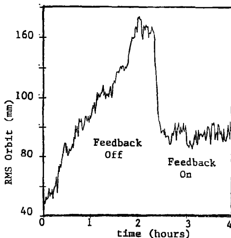
Figure 4. Example of SVD orbit control on SPEAR.
