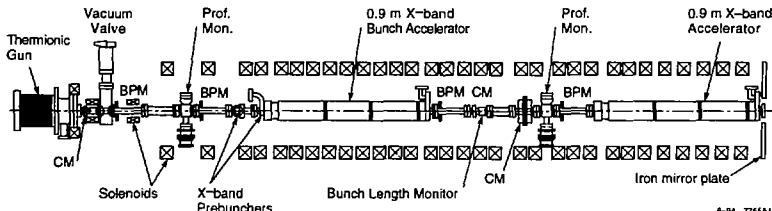
Fig. 1. The NLCTA Injector layout.
