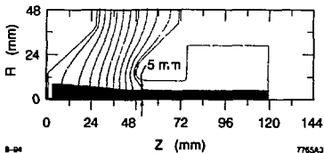
Fig. 2. Beam envelope from the NLCTA thermionic gun.
