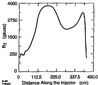
Fig. 3. Axial magnetic field along the NLCTA injector.
