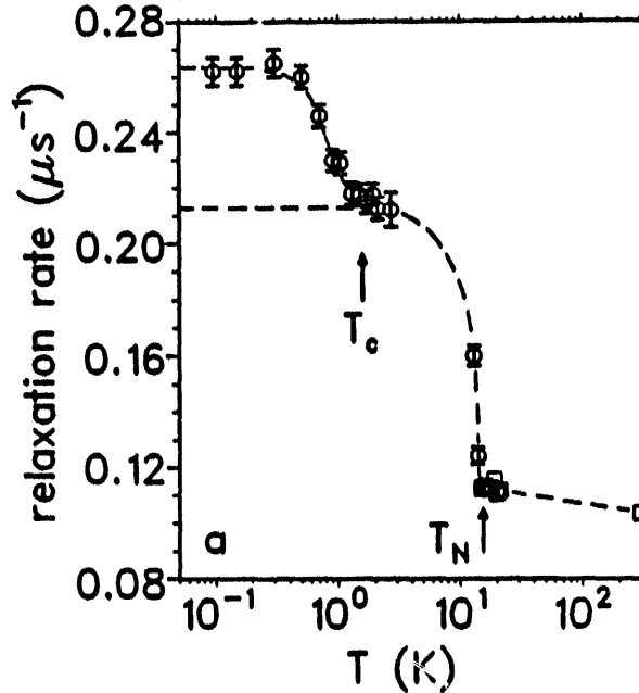
Fig. 1. The \mu SR relaxation rate for \text{UPd}_2\text{Al}_3 in transverse applied field of 340 G for T < 10\text{K} and 117 G for T > 10\text{K} . ○ - exponential rate; □ - Gaussian rate (corrected by 1/\sqrt{2} to allow comparison. From Ref. 6.
