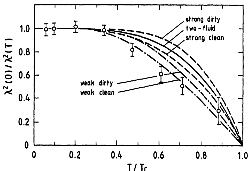
Fig. 2. The temperature dependence of the inverse-square magnetic field penetration depth in UPd_2Al_3 compared to various models for the superconducting state. From Ref. 6.
