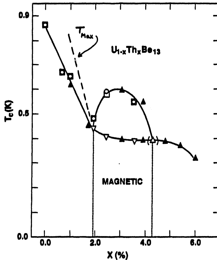
Fig. 3. Phase diagram for U 1-x Th x Be 13 . The various symbols represent different types of measurements, explained in Ref. 8. The dotted line shows the approximate Th-dependence of the resistivity maximum T_{Max} .
