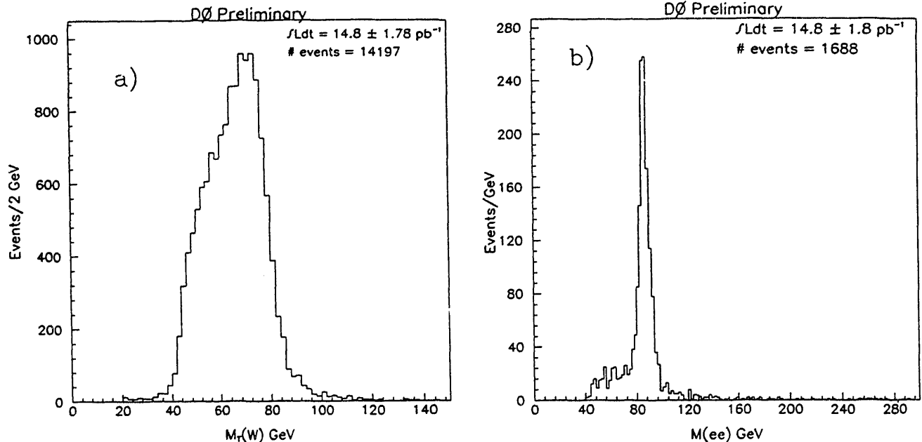
Figure 3: (a) Transverse mass distribution for W \rightarrow e\nu events and (b) Invariant mass distribution for Z \rightarrow ee events from DØ.
