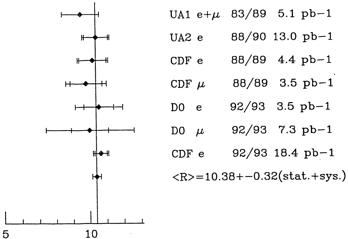
Figure 5: Compilation of R = \sigma Br(W \rightarrow \ell\nu)/\sigma Br(Z \rightarrow \ell\ell) measurements.
