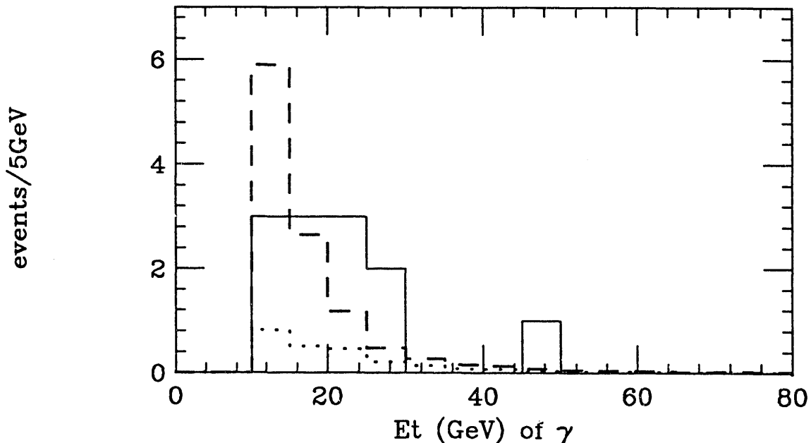
Figure 8: E_T distributions of photons (solid line) in W\gamma candidates from D\bar{O} with estimated fake photons (dotted line) and the Standard Model prediction (dashed line).
