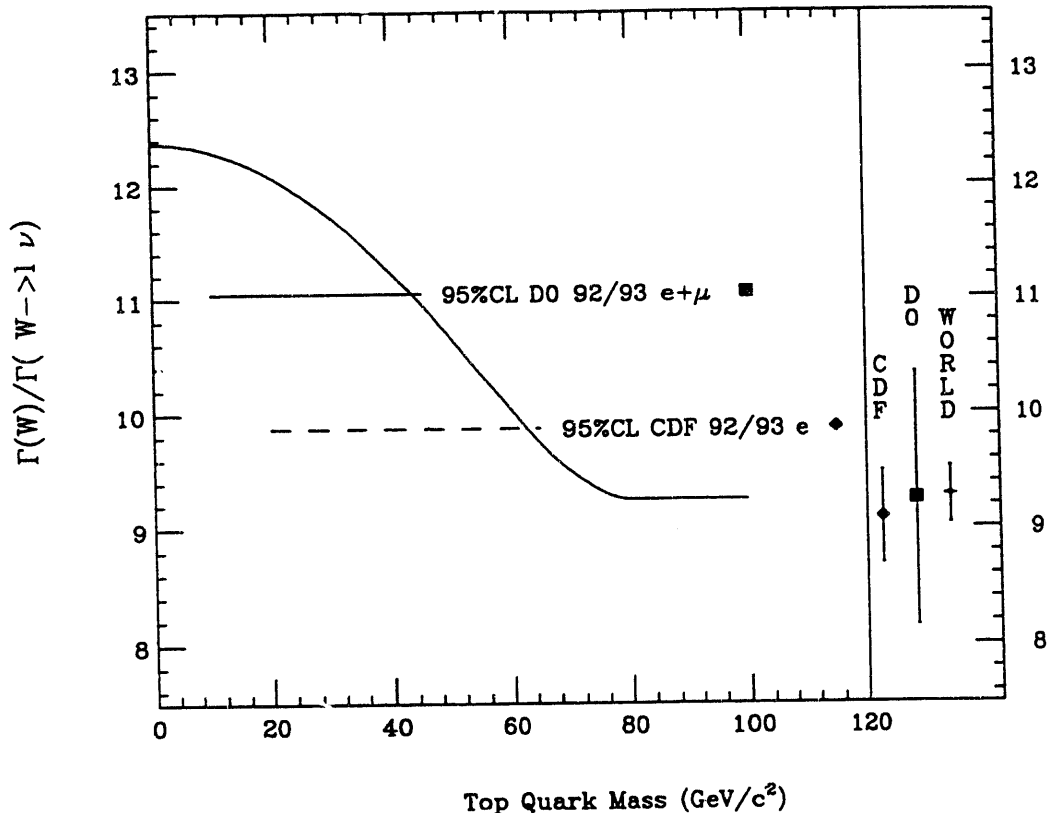
Figure 6: The ratio \Gamma(W)/\Gamma(W \rightarrow \ell\nu) as a function of the top quark mass for M_W = 80.0 \text{ GeV}/c^2 and \alpha_s = 0.13 . Also shown are preliminary measurements and the 95% C.L. limits from CDF and DØ and the average over all measurements.
