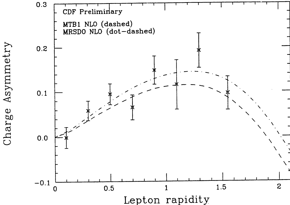
Figure 7: Charge asymmetry in W \rightarrow e\nu events from CDF. Superimposed with the data points are the predictions of MTB1 NLO (dashed) and MRSD0 NLO (dot-dashed) parton density functions.
