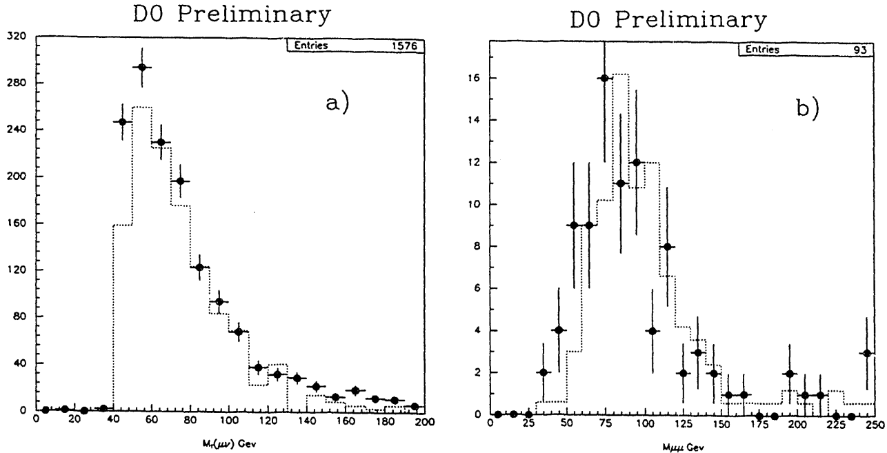
Figure 4: (a) Transverse mass distribution for W \rightarrow \mu\nu events and (b) Invariant mass distribution for Z \rightarrow \mu\mu events from D\bar{D} . In both figures the points are the data and the dotted line is the Monte Carlo prediction for the signal.
