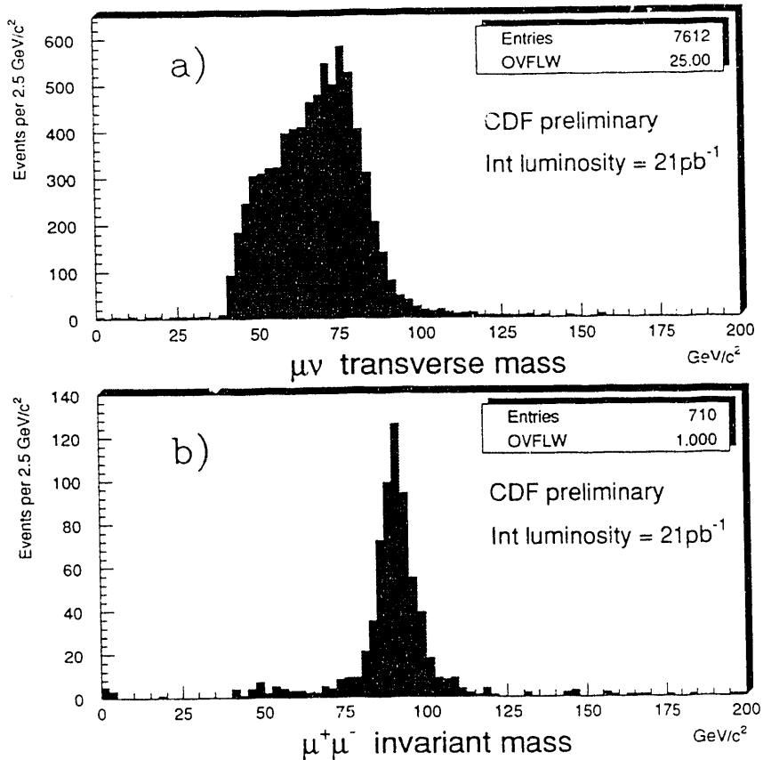
Figure 2: (a) Transverse mass distribution for W \rightarrow \mu\nu events and (b) Invariant mass distribution for Z \rightarrow \mu\mu events from CDF.
