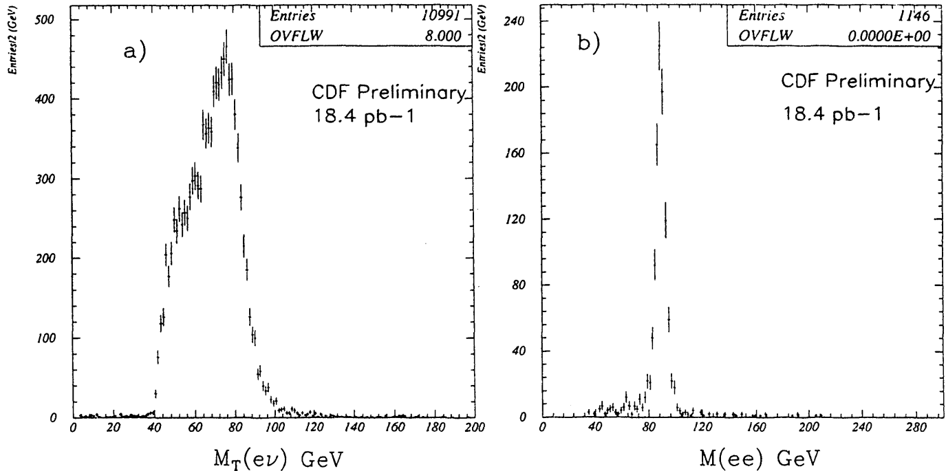
Figure 1: (a) Transverse mass distribution for W \rightarrow e\nu events and (b) Invariant mass distribution for Z \rightarrow ee events from CDF.
