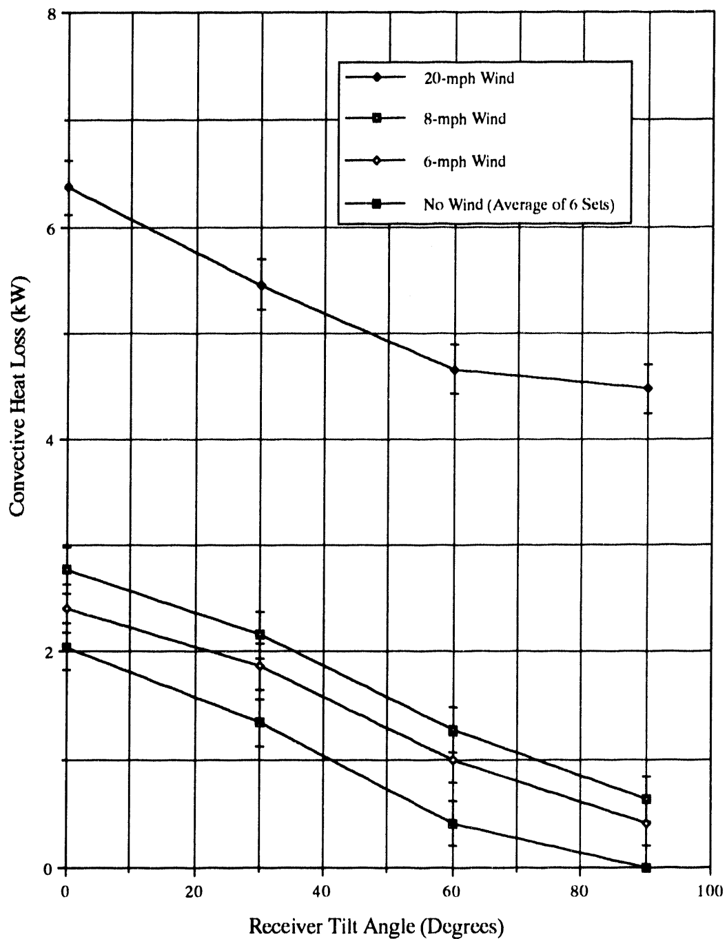
Figure 8. Convective heat loss from receiver at 530°F for side-on winds of various speeds.
