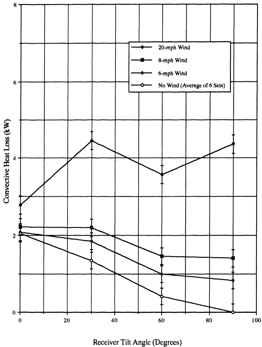
Figure 9. Convective heat loss from receiver at 530°F for head-on winds of various speeds.
