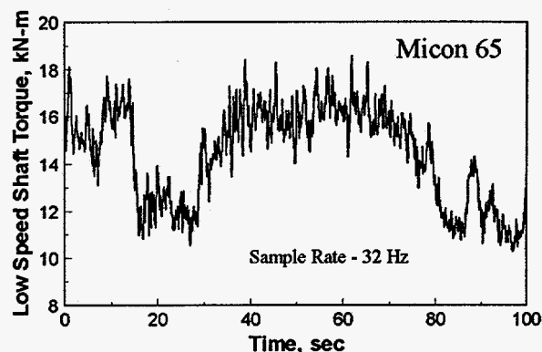
Figure 2. Typical Time Series Data for the Low Speed Shaft Torque on the Micon 65.
