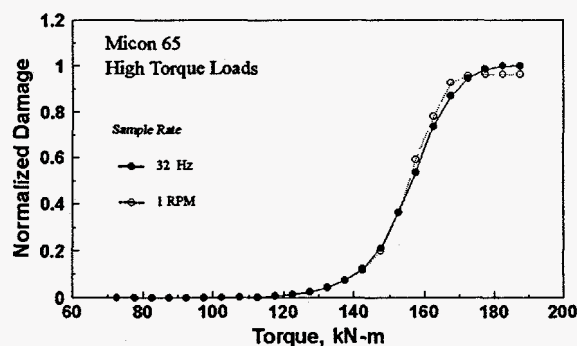
Figure 8. Accumulated Damage for the Pinion Gear on the Micon 65.
