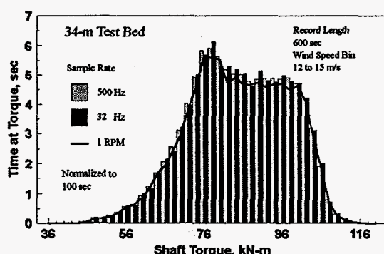
Figure 7. Time-at-Torque Histogram for the Test Bed.
