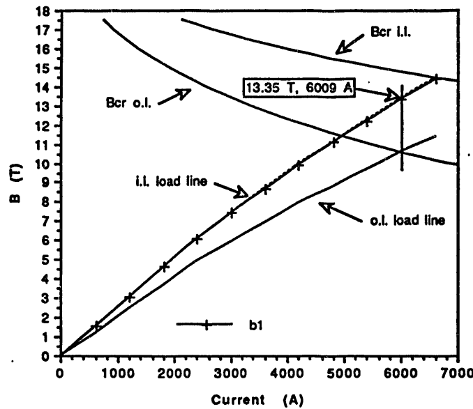
Figure 3: Load lines and short sample curves
