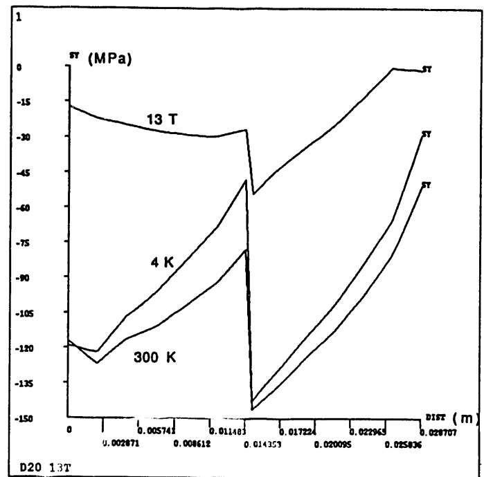
Figure 6: Azimuthal stress at the inner layer pole
