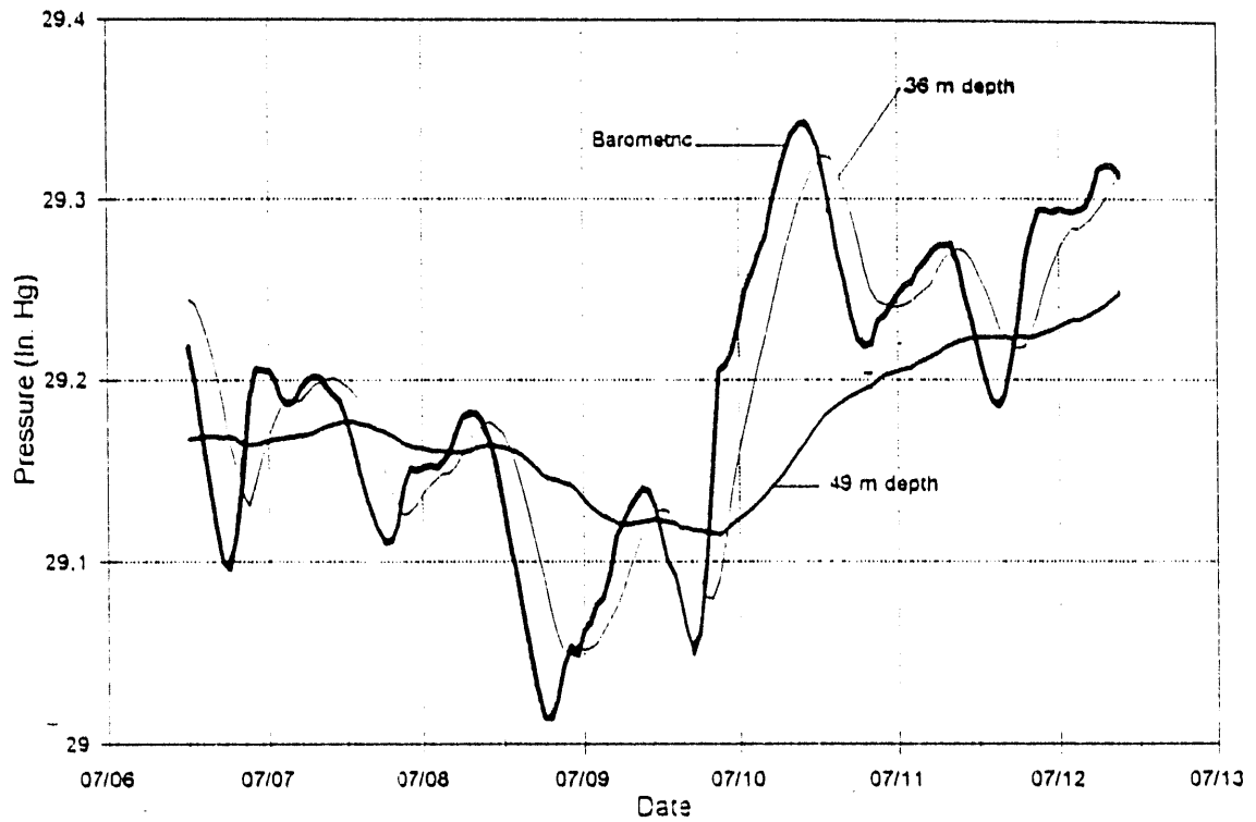
Figure 4. Effect of Relatively Impermeable Layer on Attenuation of Barometric Pressure Wave at Hanford's Well 299-W18-247 (4a) and at Savannah River's Well MHV1 (4b).
