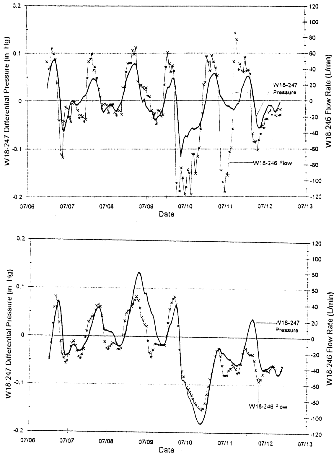
Figure 6. Differential Pressure and Flow Rate Above (6a) and Below (6b) the Caliche in Hanford's Wells 299-18-246 and 299-W18-247. A positive (+) flow rate denotes soil gas flow to the atmosphere and a negative (-) flow rate denotes inflow of ambient air to the subsurface.
