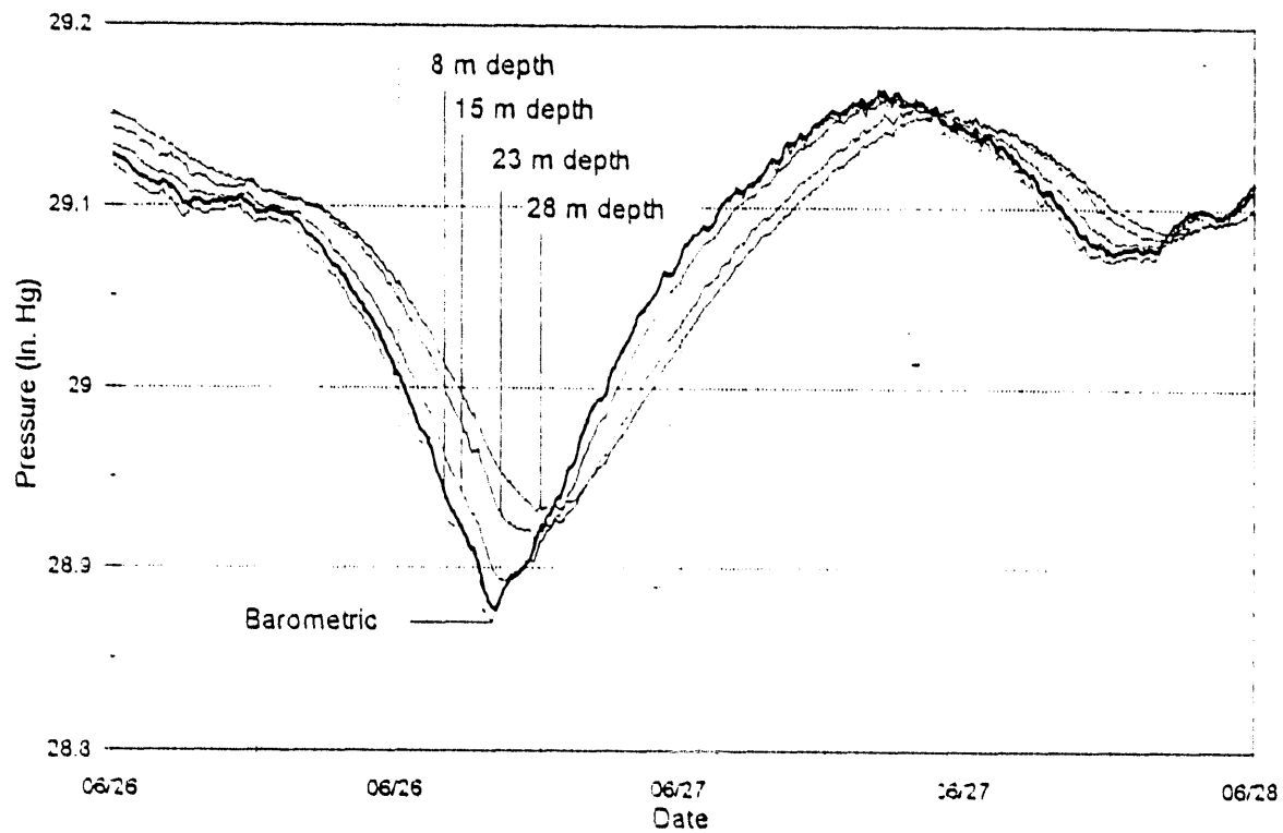
Figure 3. Barometric Pressure and Subsurface Soil-Gas Pressures Measured at Hanford Station "CPT4" (3a) and at Savannah River Station "MVC-3" (3b).
