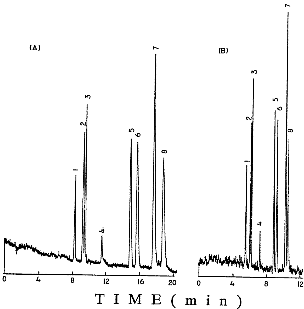
Fig. 6. Influence of a step change in [CTAB] on the separation of organic anions. Before injection, the concentration of CTAB is 4\ \mu\text{M} while the running concentrations are 10\ \mu\text{M} for A and 40\ \mu\text{M} for B, respectively. Conditions are the same as those in Fig. 4.
