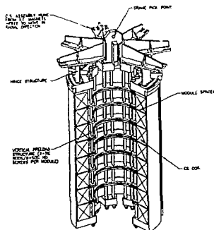
Fig. 4. Central Solenoid Assembly
