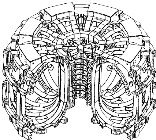
Fig. 1. TPX Superconducting Magnet System
