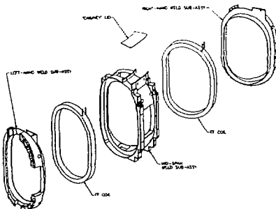
Fig. 3. TPX Module consisting of two coils, case and internal structure
