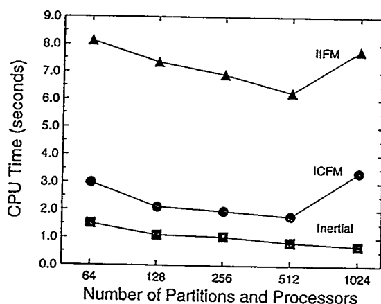
FIG. 2. Partition time for the CVD grid on the Paragon.
