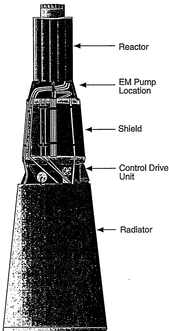
Figure 2. The Topaz II Power System.
