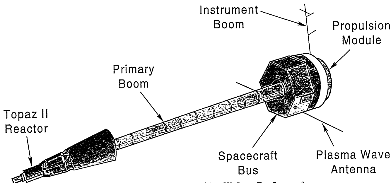
Figure 1. Orbital Configuration of the NEP Space Test Spacecraft.
