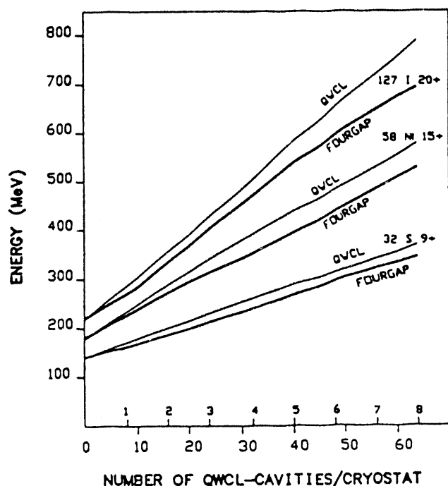
Figure 2. Energy gain versus the number of QWCL-cavities. Each cryostat will have 8 single or 4 coupled QWCL-cavities. The upper number on the x-axis shows the number of cryostats.
