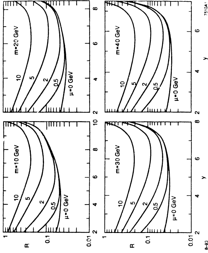
The ratio R(\mu) as a function of y , at \bar{y} = 0 .
