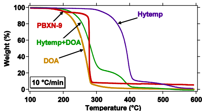
Figure 3. TGA results for PBXN-9, Hytemp, DOA, and Hytemp + DOA
