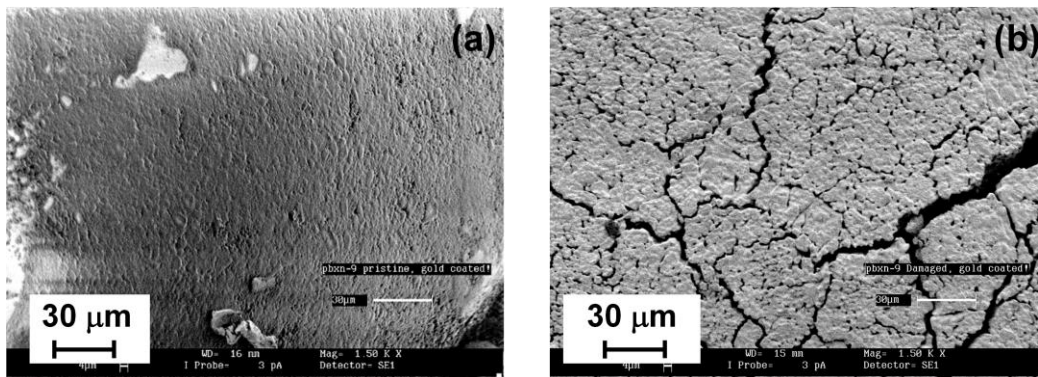
Figure 12. Microscopic pictures of pressed part, (a) before and (b) after heating for 3 hours at 180 °C.
