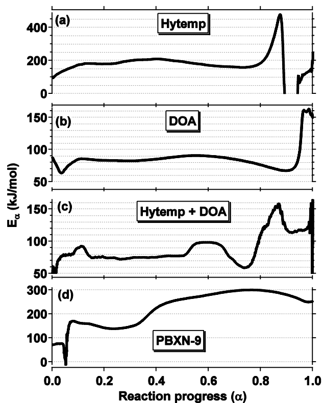
Figure 6. Decomposition kinetics from the isoconversional analysis of TGA data for (a) Hytemp 4454 (b) DOA (c) Hytemp + DOA and (d) PBXN-9.
