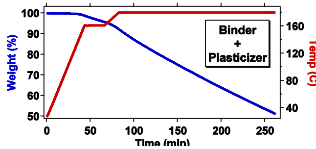
Figure 14. Thermogravimetric results of binder + plasticizer (Hytemp + DOA) under thermal conditions similar to those used in the thermal damage experiments (i.e. 3 hrs at 180 °C).
