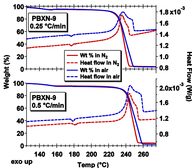
Figure 5. Weight loss and heat flow results for PBXN-9 in air and N 2 atmosphere.
