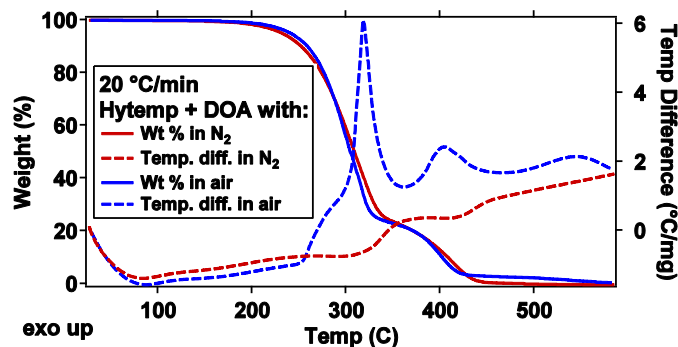
Figure 4. TGA and DTA results for Hytemp + DOA in air and N 2 atmosphere.
