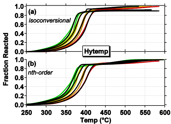
Figure 7. Comparison of (a) isoconversional and (b) n^{\text{th}} -order predictions with raw data for the decomposition of Hytemp; colored lines are raw data, black lines are fit-predictions.
