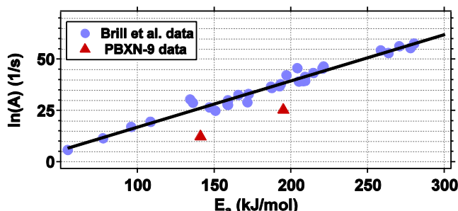
Figure 11. HMX thermal decomposition kinetic compensation plot. Brill et al. data from Table 1 in reference [17].
