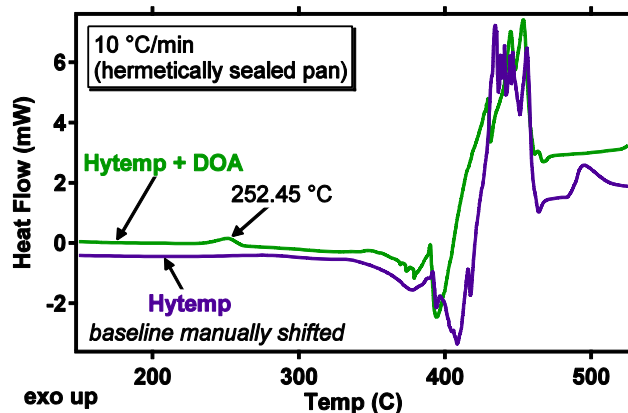
Figure 2. DSC results for Hytemp and Hytemp + DOA
