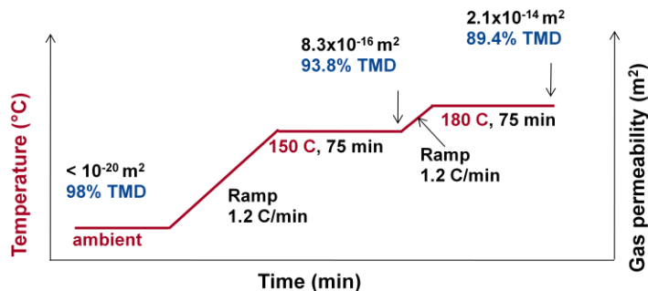
Figure 15. Gas permeability and bulk density at various temperatures for the radially confined PBXN-9 specimen. Densities are calculated based on results of low-density pristine samples reported in Table 5.
