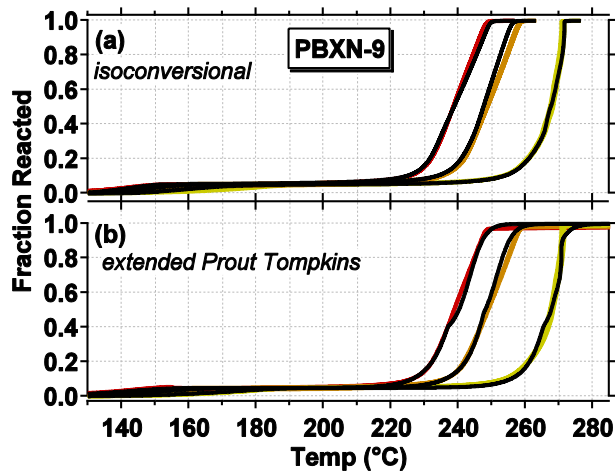
Figure 10. Comparison of (a) isoconversional and (b) extended-Prout-Tompkins (3-stage model) predictions with raw data for the decomposition of the PBXN-9; colored lines are raw data, black lines are fit-predictions.
