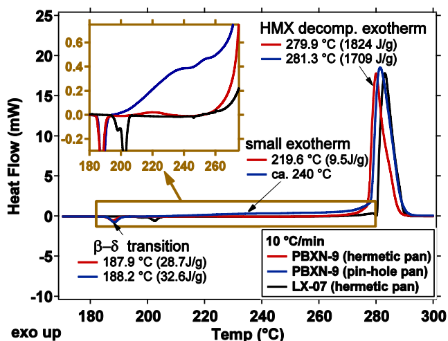
Figure 1. DSC results for PBXN-9 and LX-07 in two different pan types.
