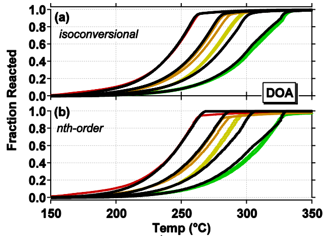
Figure 8. Comparison of (a) isoconversional and (b) n^{\text{th}} -order predictions with raw data for the decomposition of DOA; colored lines are raw data, black lines are fit-predictions.
