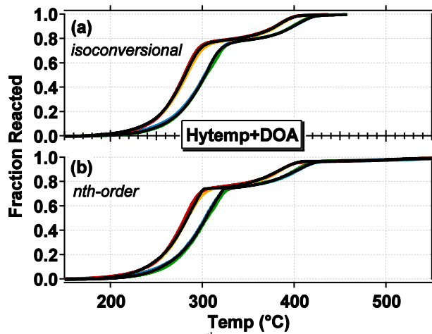
Figure 9. Comparison of (a) isoconversional and (b) n^{\text{th}} -order predictions with raw data for the decomposition of the mixture Hytemp + DOA; colored lines are raw data, black lines are fit-predictions.
