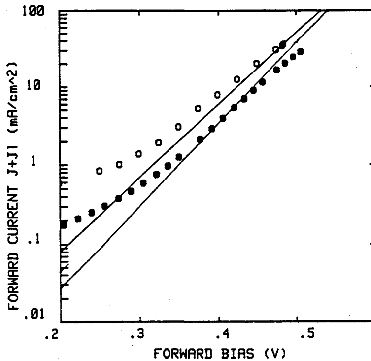
Fig. 12. Logarithmic plot of J+J_1 (□) and dark I-V (■) characteristics of the device of Fig. 10. Solid lines represent data corrected for R_s ( 0.2 and 0.3 \Omega\text{-cm}^2 in light and dark, respectively).
