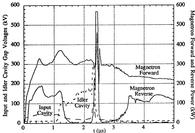
Fig. 5: Input and idler cavity gap voltages and magnetron power for shot 1308.
