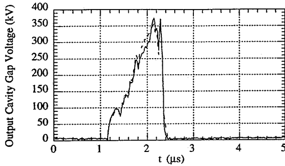
Fig. 4: Output cavity gap voltage for shot 1308.
