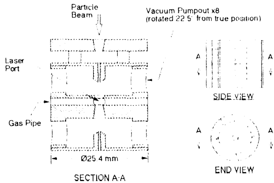
Figure 3: Plasma Chamber
