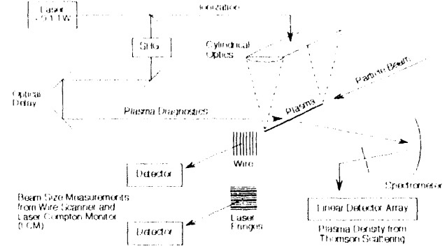
Figure 1: Outline of Plasma Lens Experimental Setup
