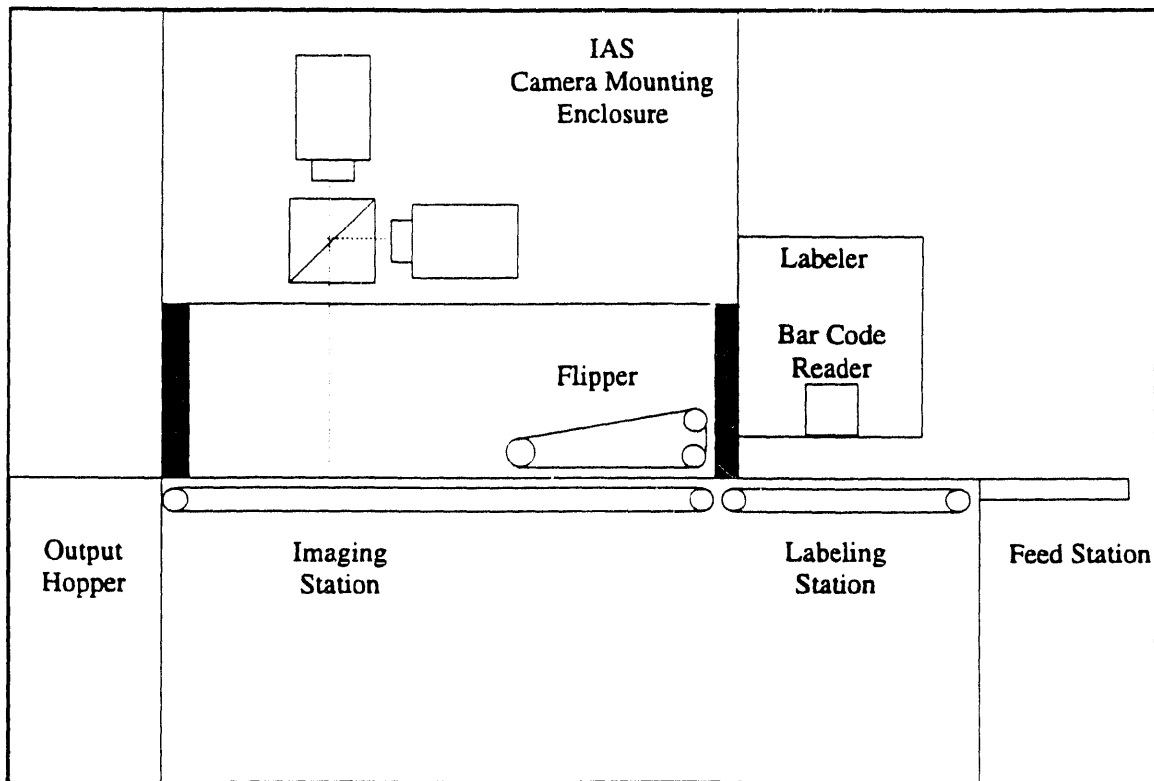
Fig. 3. The CIS and IAS hardware layout.
