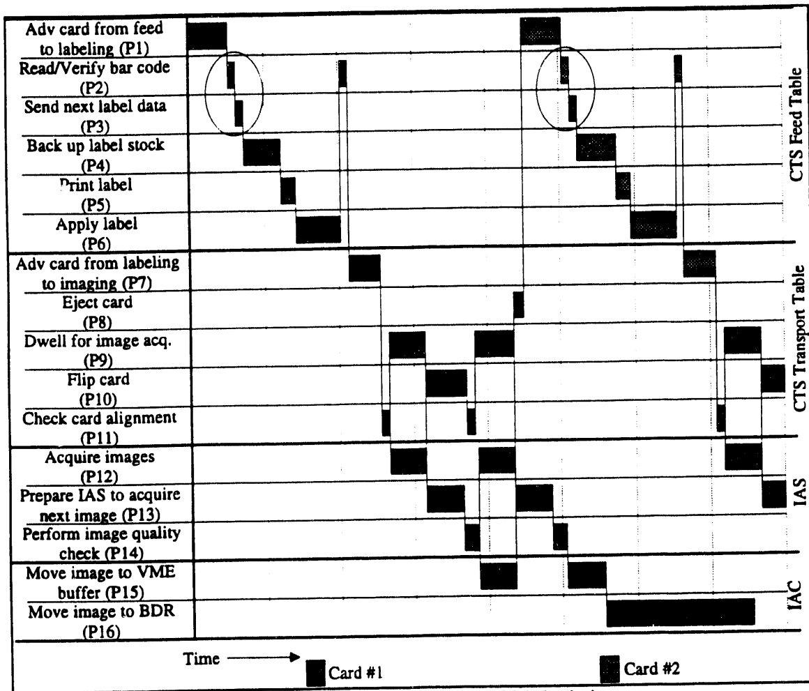
Fig. 10. Implementation of on-demand label printing.
