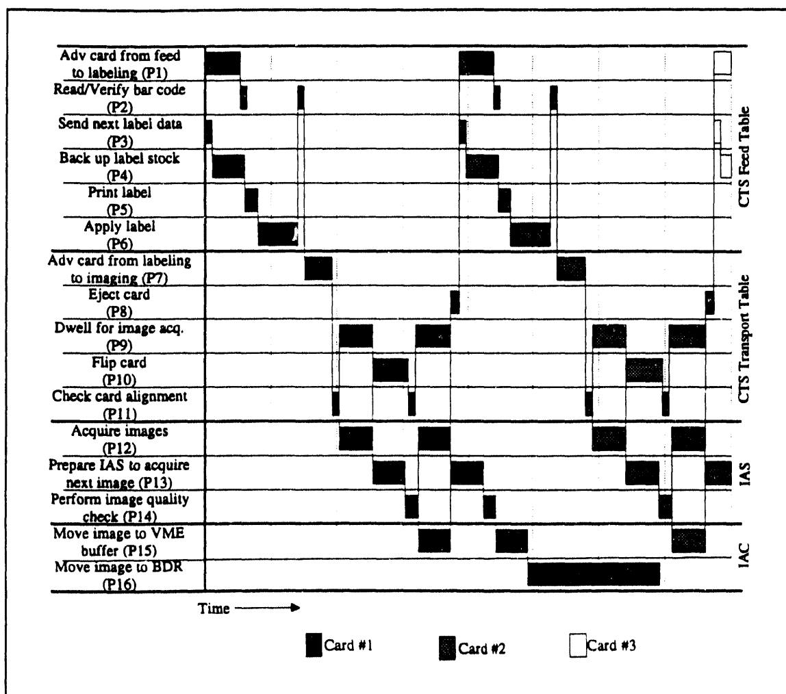
Fig. 5. A timing diagram for the HSFE.
