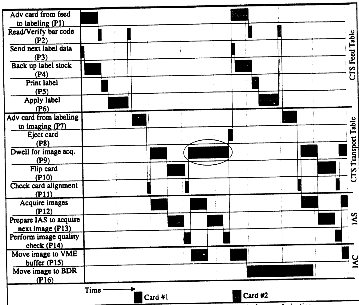
Fig. 9. Implementation of image quality check completion before card ejection.
