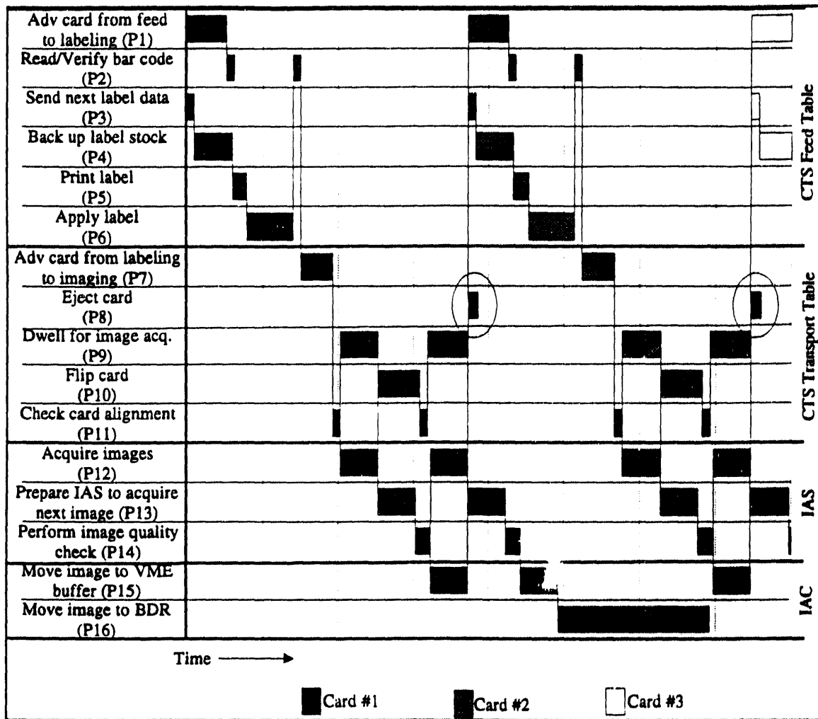
Fig. 7. Implementation of simultaneous card ejection and card advance.
