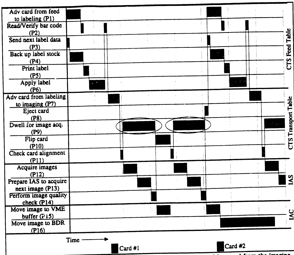
Fig. 8. Implementation of image quality check completion before the card is moved from the imaging station.
