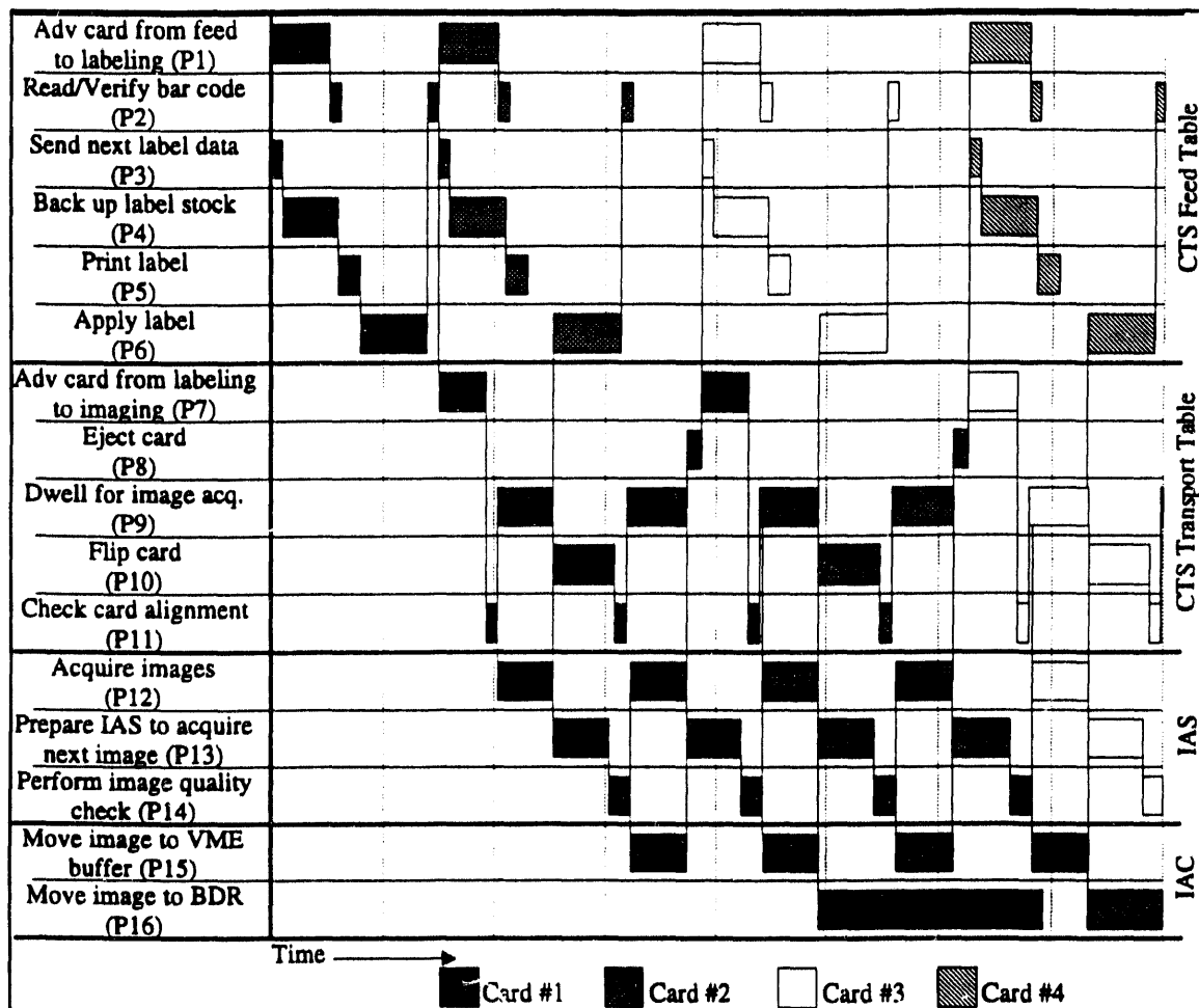
Fig. 12. Implementation of concurrent labeling and imaging operations.
