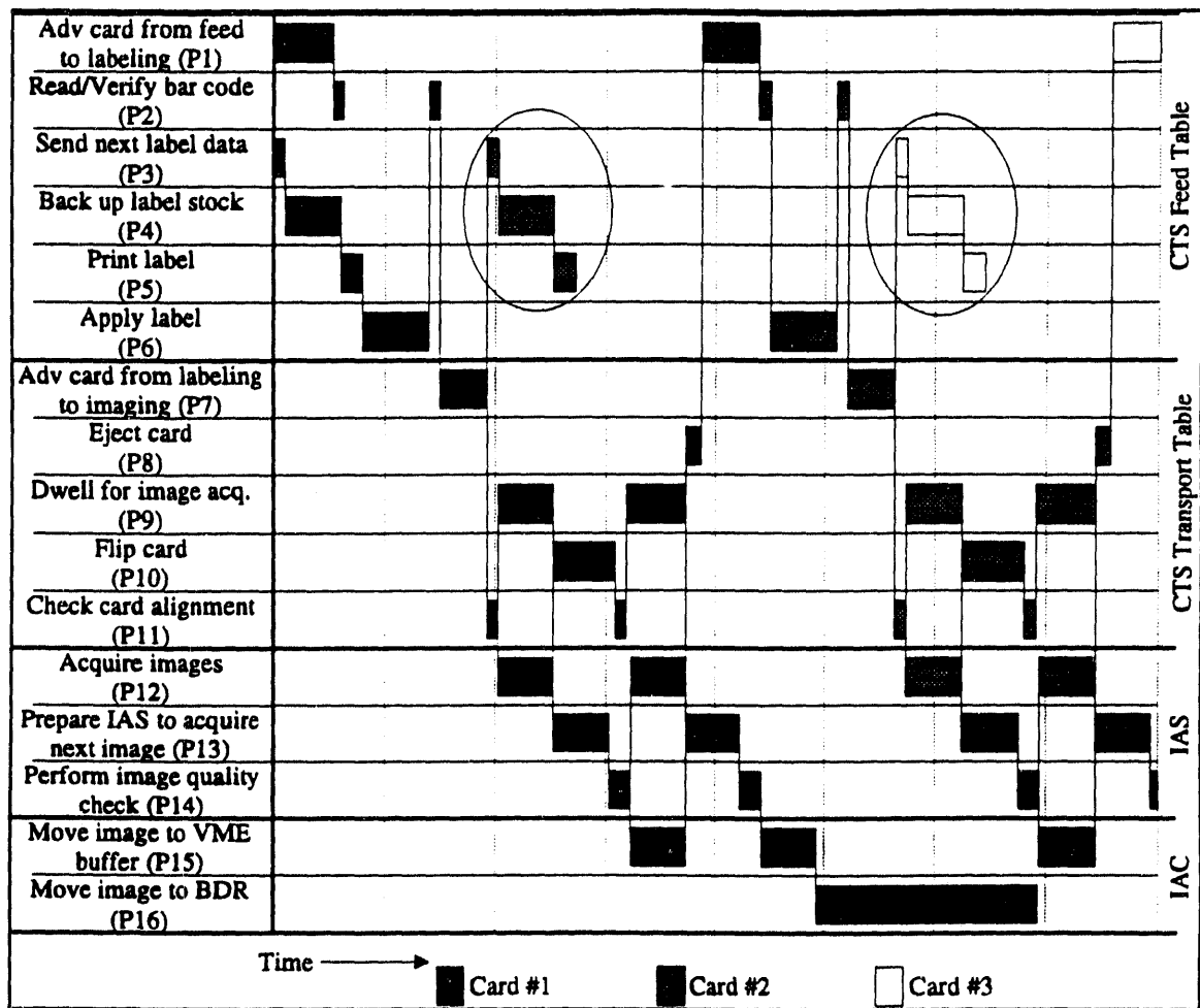
Fig. 11. Implementation of label printing for the next card during imaging of the current card.
