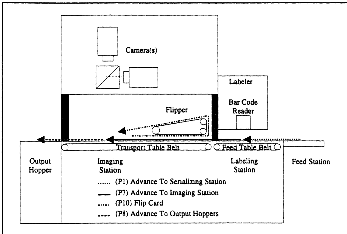
Fig. 6. The three belts controlling card motion in the HSFE.
