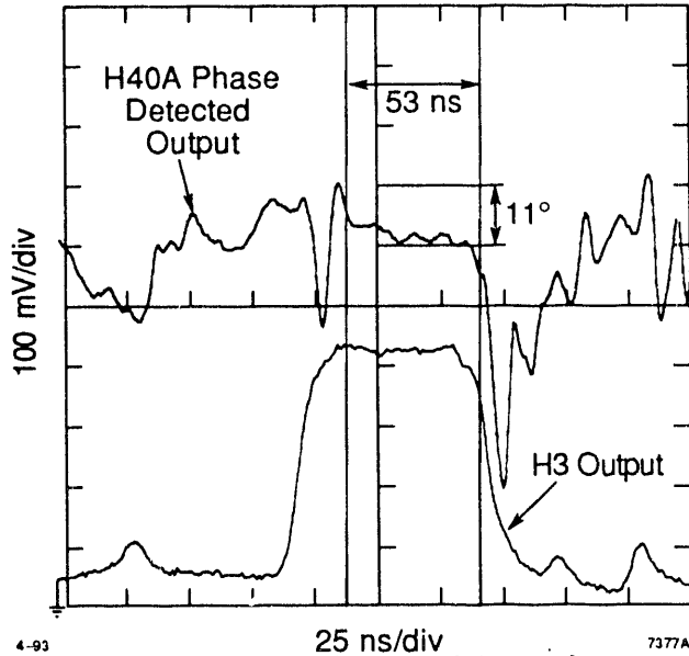
Figure 7. Amplitude and phase of the combiner output pulse.
