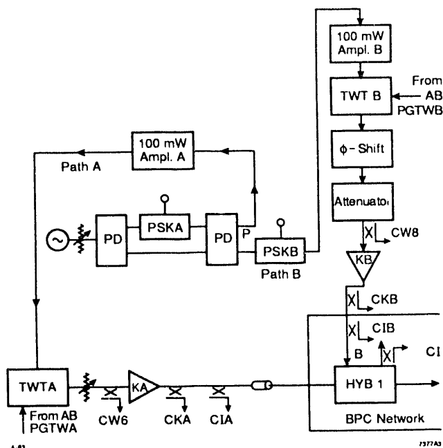
Figure 3. Two-klystron BPC drive system.
