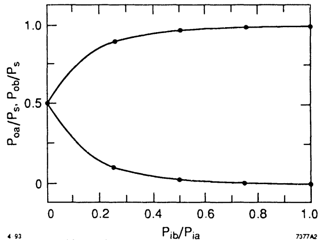
Figure 2. Normalized output powers vs. input power ratio.
