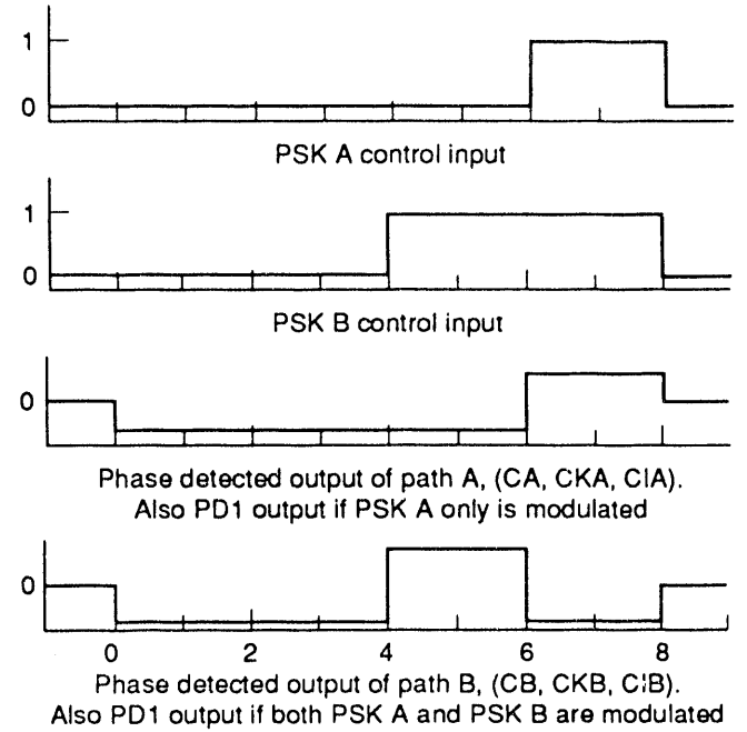
Figure 8. Two-stage BPC modulation (horizontal unit = 70 ns).
