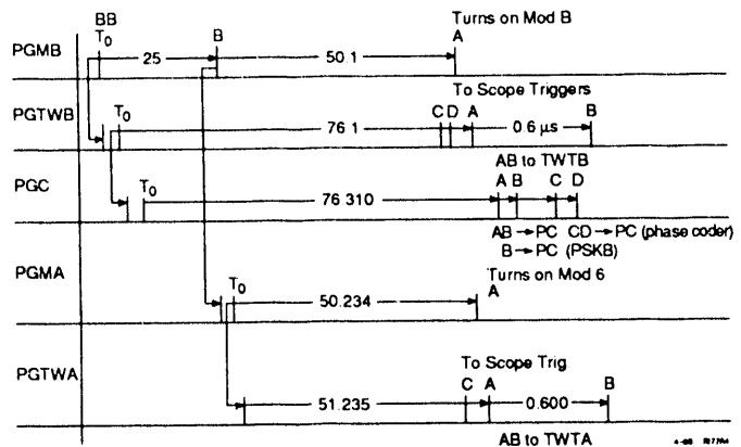
Figure 4. Timing and triggering.
