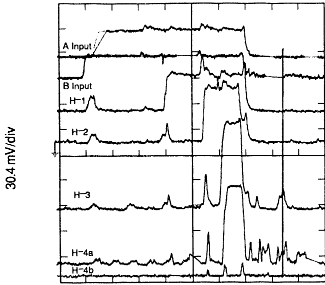
Figure 6. 3-stage BPC outputs.
