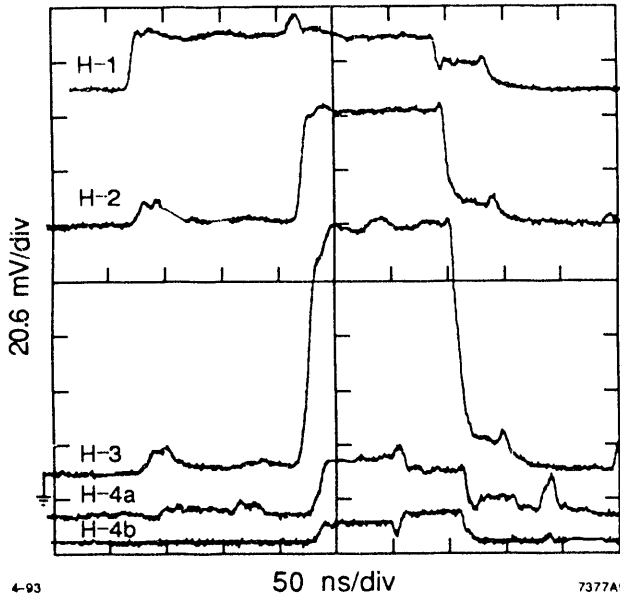
Figure 9. Two-stage BPC outputs.
