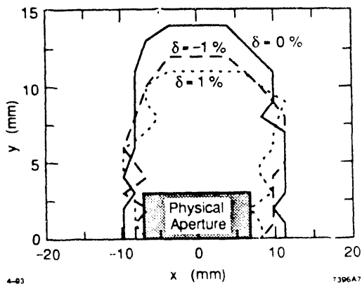
Fig. 4 Dynamic aperture in the new damping ring design at the injection point for initial energy deviations of 0% and \pm 1\% . Particles were tracked for 1000 turns with synchrotron oscillations and alignment errors.
