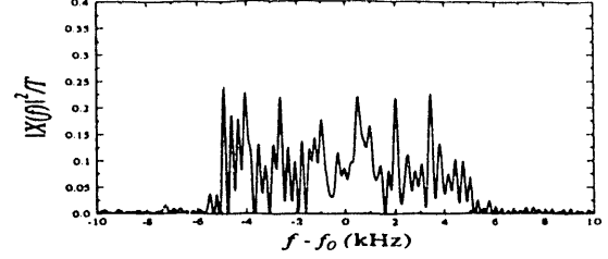
Figure 2: Power spectrum for the input signal x(t) .
