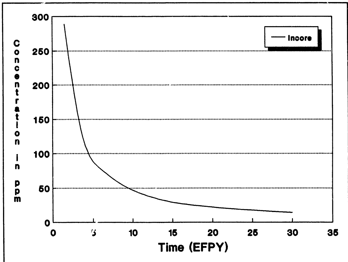
Figure 14. Niobium concentrations in inconel which will cause Nb-94 to exceed its Class C limit as a function of time. ( \phi=1 \times 10^{13} neutrons/cm 2 -sec.)
