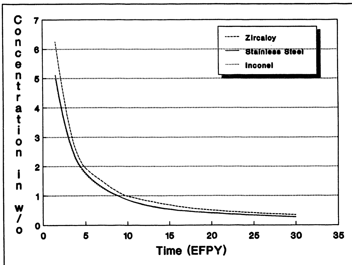
Figure 7. A comparison of the allowable initial nickel concentrations for various irradiation times in zircaloy, stainless steel, and inconel. ( \phi=1 \times 10^{13} neutrons/cm 2 -sec.)
