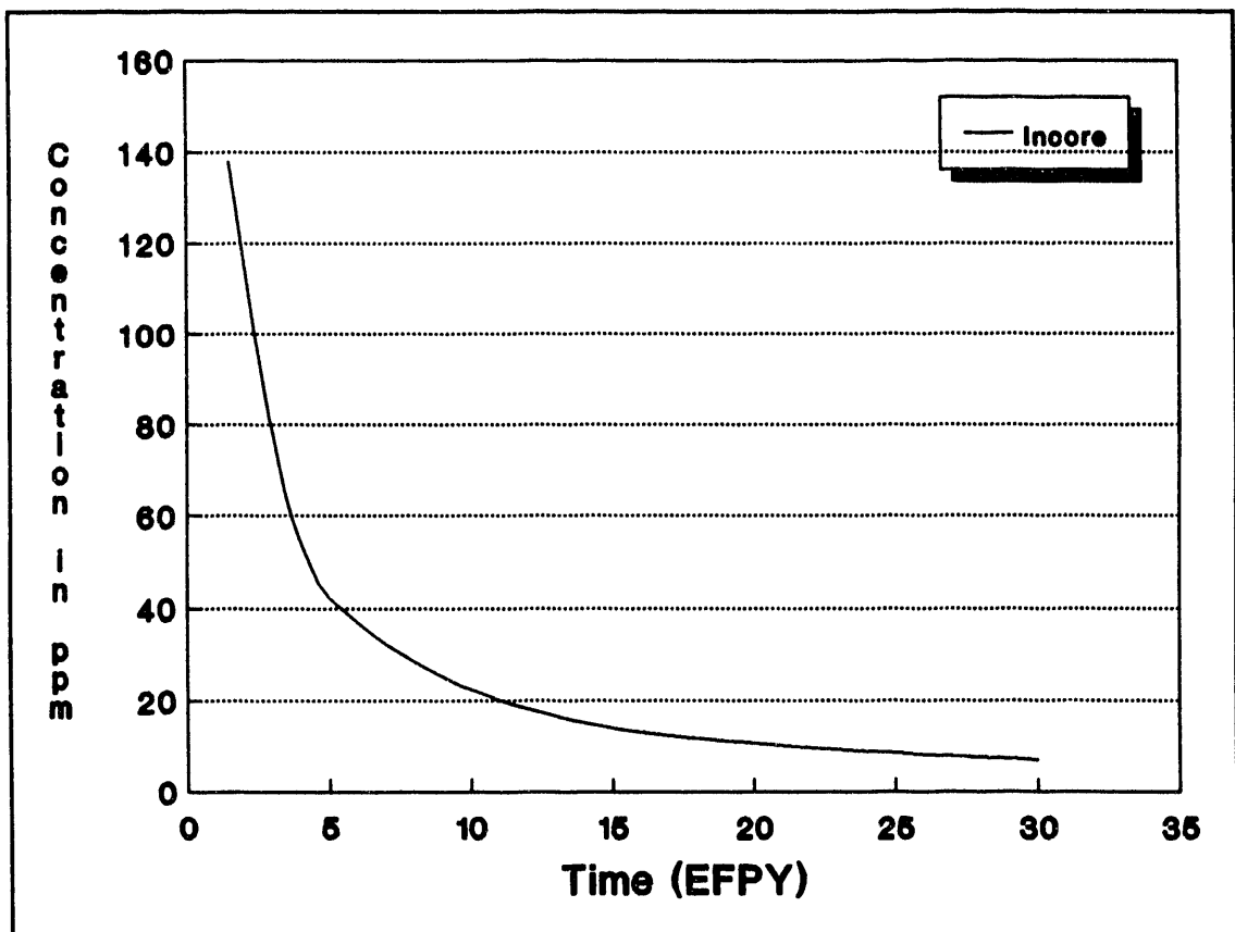
Figure 8. Niobium concentrations in inconel which will cause Nb-94 to exceed its Class C limit as a function of time. ( \phi=1 \times 10^{13} neutrons/cm 2 -sec.)
