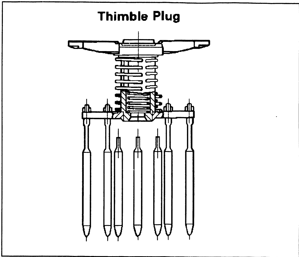
Figure 4. Westinghouse Thimble Plug Assembly.
