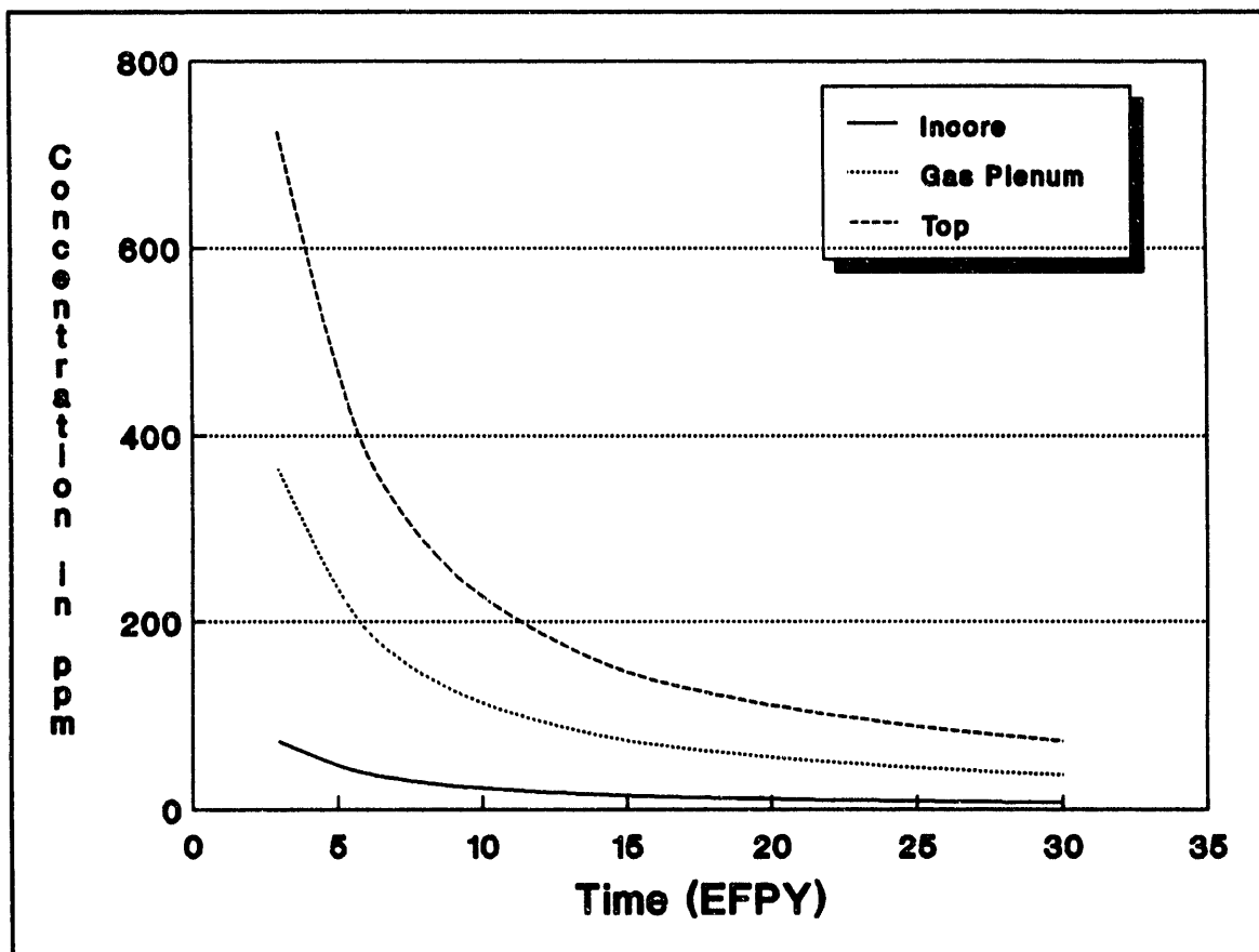
Figure 11. Allowable initial niobium concentrations in stainless steel as a function of irradiation time for three different vertical positions in the core.
