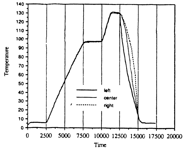
Figure 4: Temperature at left, center, and right top edge of lower block as a function of time. Note the dramatic influence of thermal contact conditions on the temperature variations.
