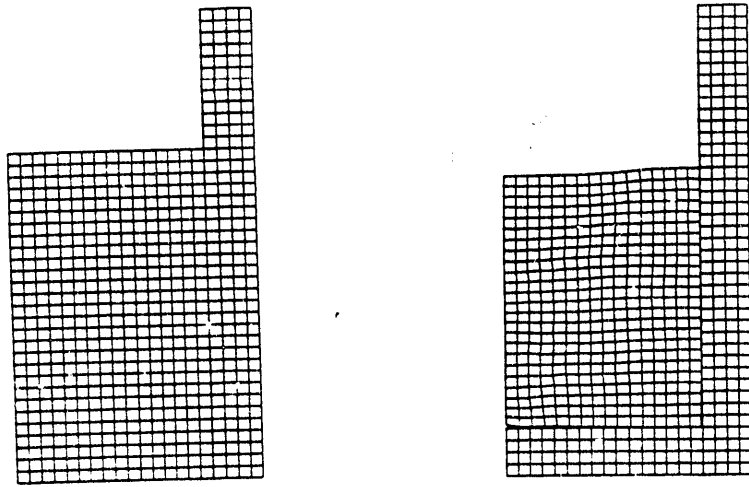
Figure 5: Axisymmetric finite element mesh on the original geometry (left) and the final geometry (right) for the solidification of an aluminum melt in a steel can.
