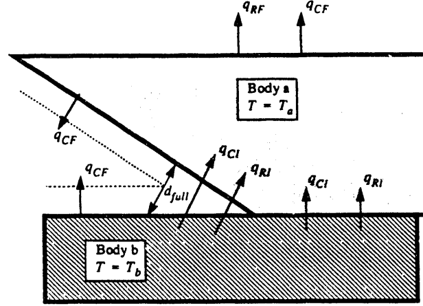
Figure 2: Schematic depiction of the thermal boundary conditions.
