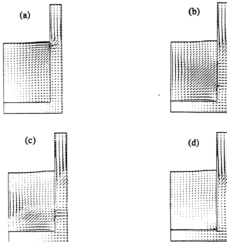
Figure 6: Time sequence of heat flux vectors showing the effect of changing contact conditions on the heat flow path.
