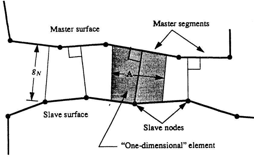
Figure 1: Discretization of the contact boundary showing the gap function g_N , the “effective one-dimensional conduction element,” and the interface element area A .
