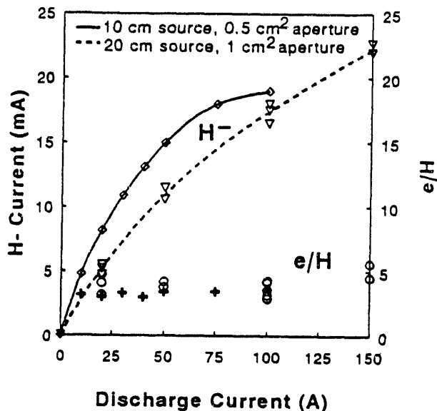
Fig. 2 - Comparison of the H - current and electron-to-H - ratio vs. discharge current for the 10 cm and 20 cm diameter BNL sources.
