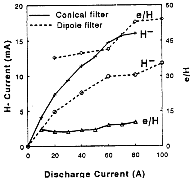
Fig. 5 - H^- current and electron-to- H^- ratio vs. discharge current for the conical and dipole filter field geometries.
