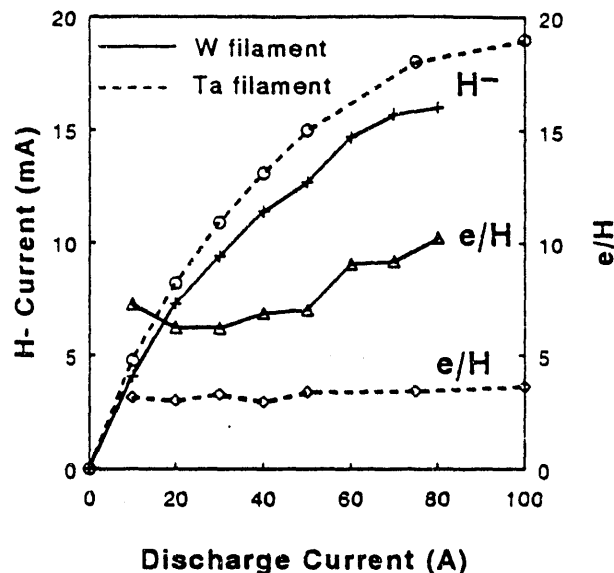
Fig. 3 - H - current and electron-to-H - ratio vs. discharge current when operating the source with tungsten and tantalum filaments.
