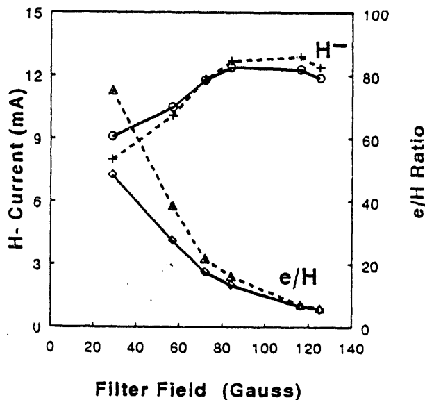
Fig. 4 - H - current and electron-to-H - ratio as a function of the strength of the conical filter field. Dotted line: plasma electrode floating; solid line: plasma electrode grounded. Discharge current = 50 A.
