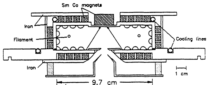
Fig. 1 - Cross section of the small BNL volume source. Magnetic field lines are shown schematically.
