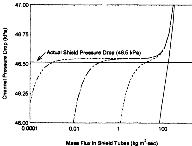
Figure 6.19. Channel Pressure Drop vs. Mass Flux in Shield Tubes
