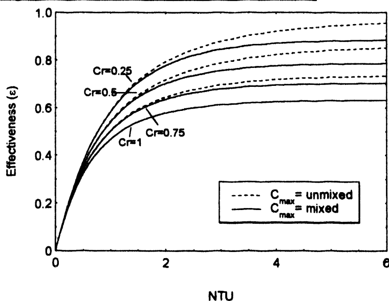
Figure 6.6. Effectiveness vs. NTU Relations
