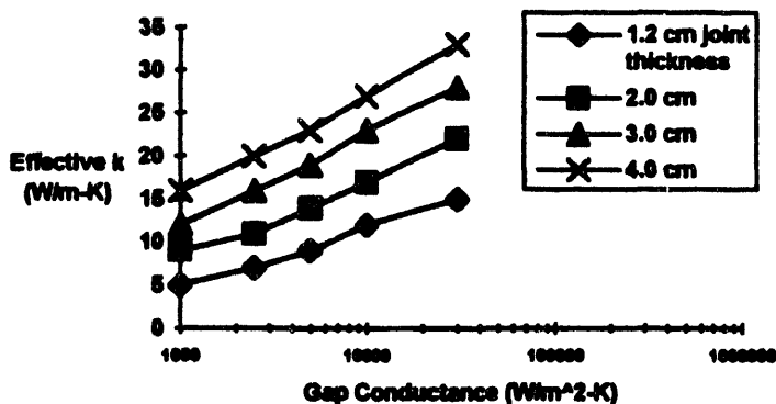
Figure 5.41. Be Joint Effective Conductivity vs. Gap Conductance (k of Be fixed at 114 \text{ W/m}\cdot\text{K} )
