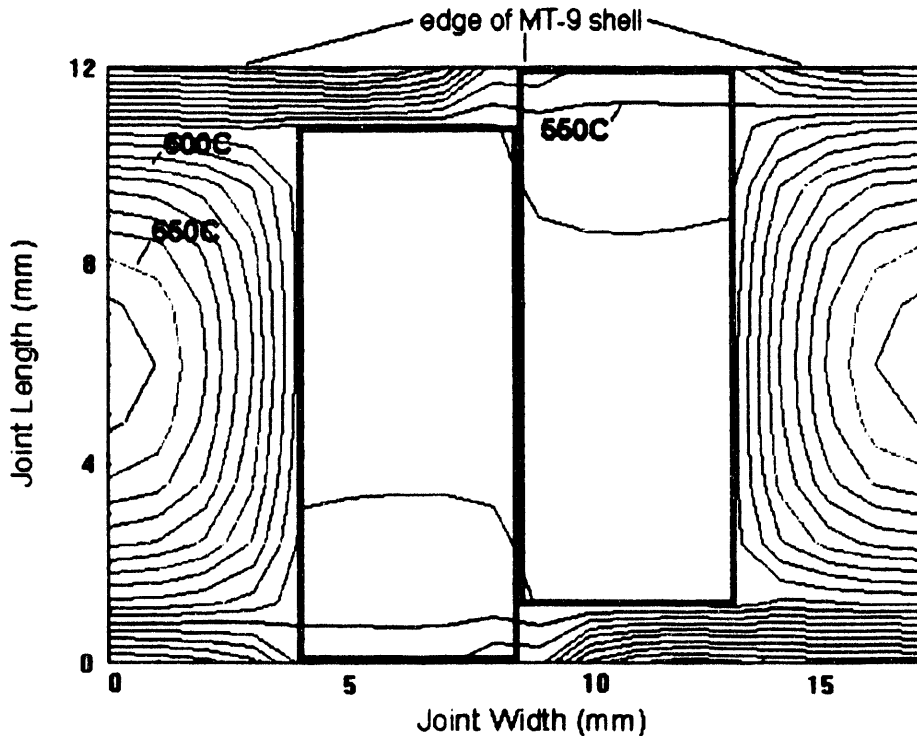
Figure 5.44. Maximum Operating Temperatures for 1st Breeder Region of Blanket Design 2
