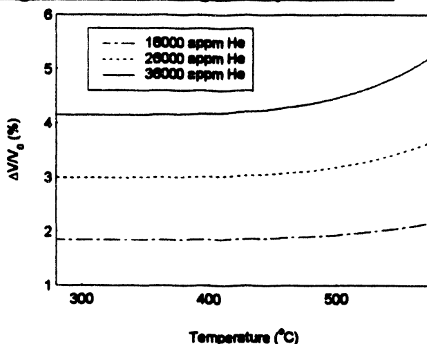
Figure 5.55. Swelling in Beryllium Slabs
