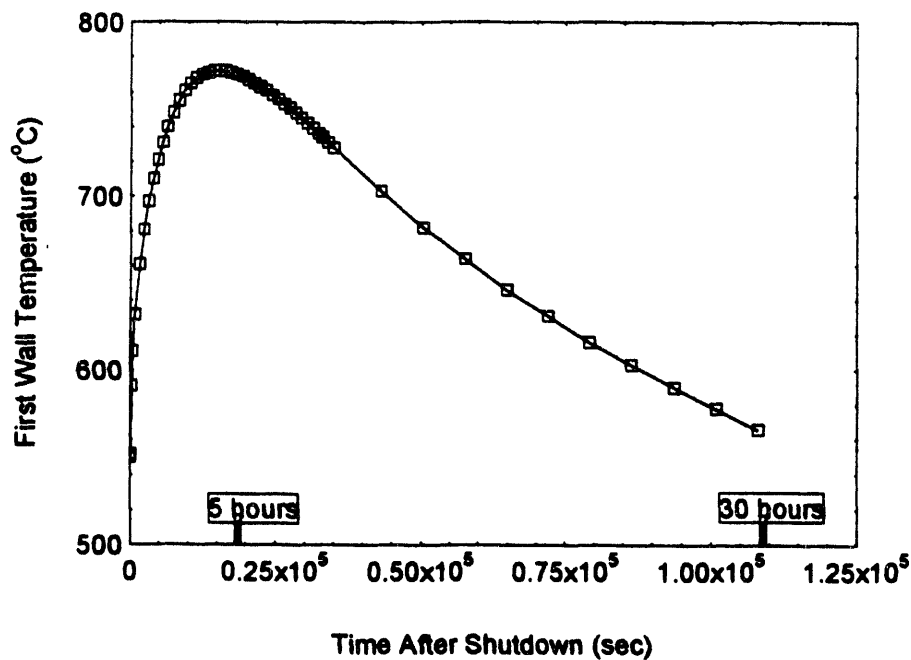
Figure 5.16. Temperature of First Wall of Blanket Design 1 After No-Flow LOFA
