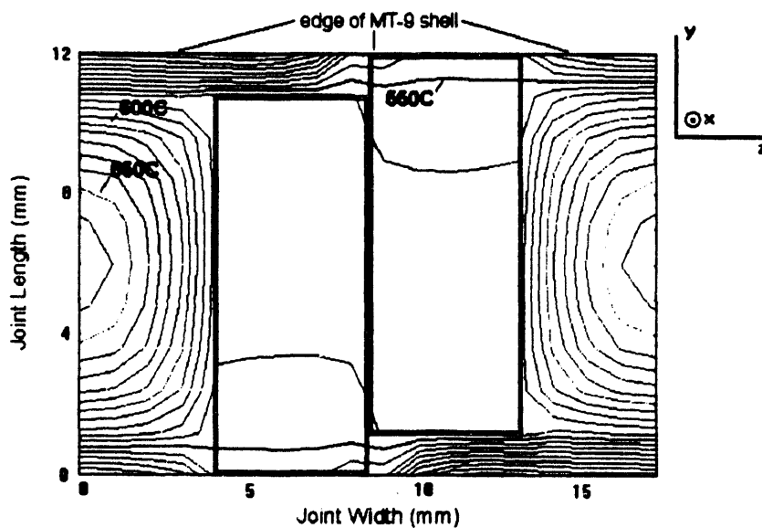
Figure 5.35. Maximum Operating Temperatures for 1st Breeder Region of Blanket Design 2
