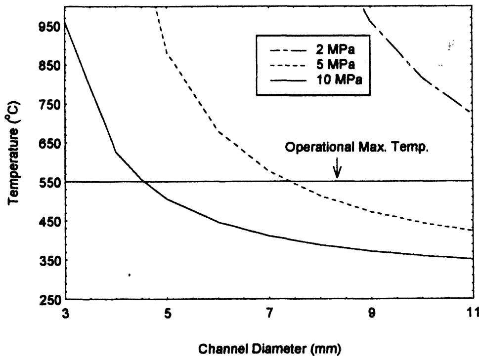
Figure 5.9. Maximum First Wall Temperatures During Natural Circulation
