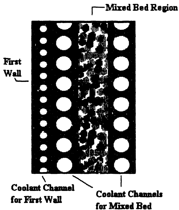
Figure 5.11. First Wall Shell Arrangement
