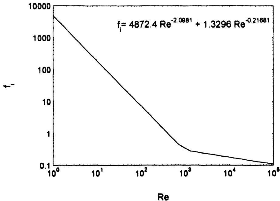
Figure 6.13. Pressure Drop Parameter for Secondary Side of Service Heat Exchanger
