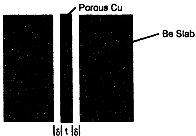
Figure 5.29. Schematic of Be/Be Gap Region
