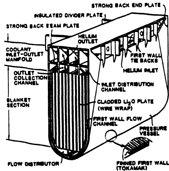
Figure 4.1. Pressurized Module Design 1
