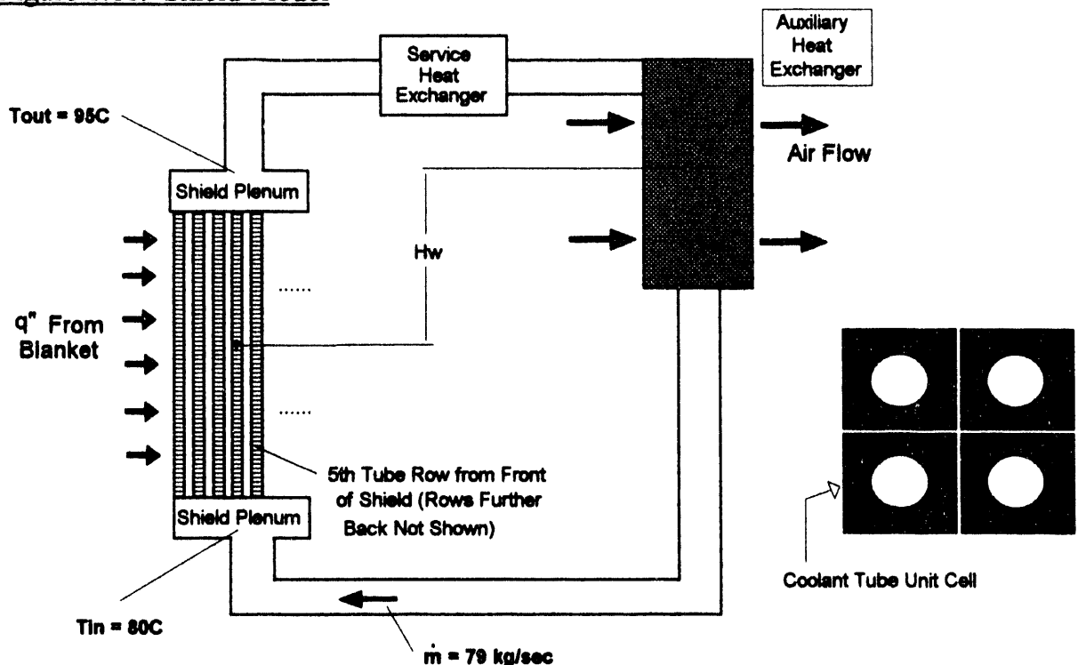
Figure 6.18. Shield Model
