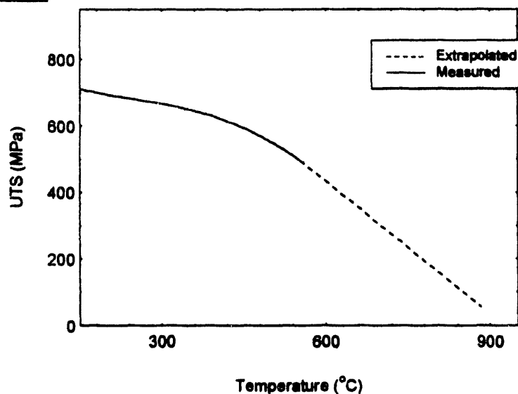
Figure 5.18. Ultimate Tensile Strength of HT/MT-9 Steel 31
