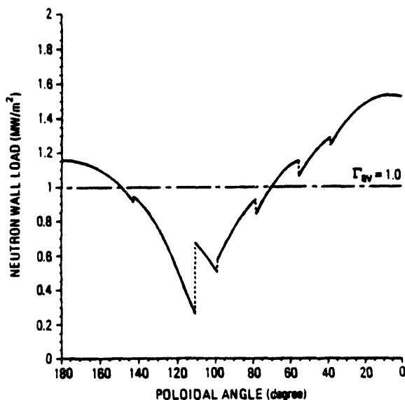
Figure 3.2. Typical Neutron Wall Load Variation 10
