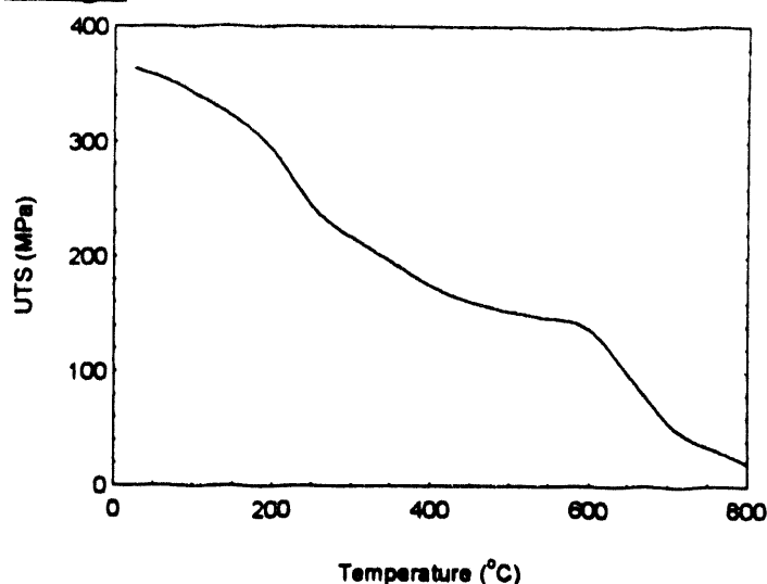
Figure 5.51. Beryllium Ultimate Tensile Strength 59
