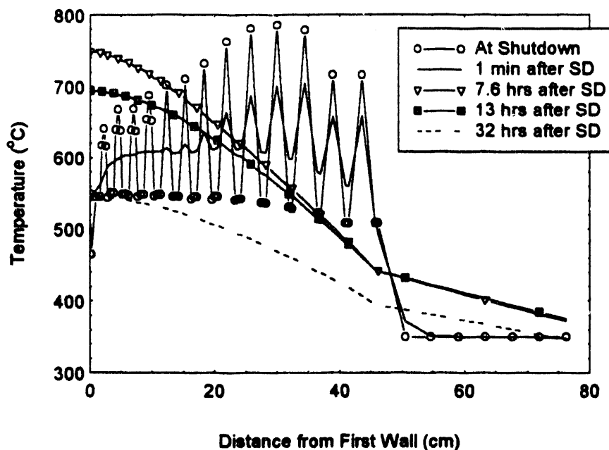
Figure 5.17. Temperatures In Blanket Design 1 After No-Flow LOFA
