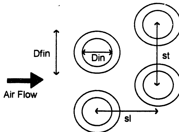
Figure 6.7. Auxiliary Heat Exchanger Fin/Tube Geometry (not to scale)
