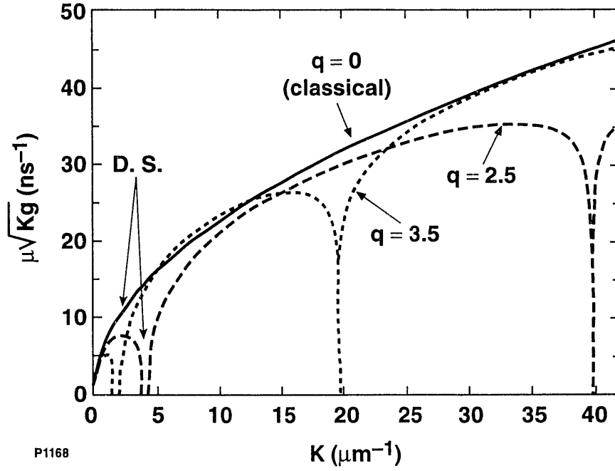
Fig. 1 Plot of the instability drive term \mu , versus the mode wave number k for modulated ( q \neq 0 ) and unmodulated ( q = 0 ) laser intensity.
