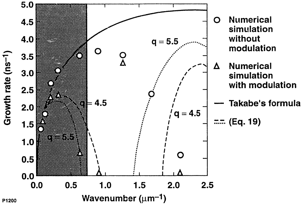
Fig. 3 Comparison of the growth rate obtained from numerical simulations (with modulation \Delta and without modulation \circ ) and the modified Eq. (19) with \alpha = 0.2 , q = 4.5 (dashed), q = 5.5 (dotted). The solid line represents Takabe formula and the shaded area represents the region with \kappa\delta < 1 .
