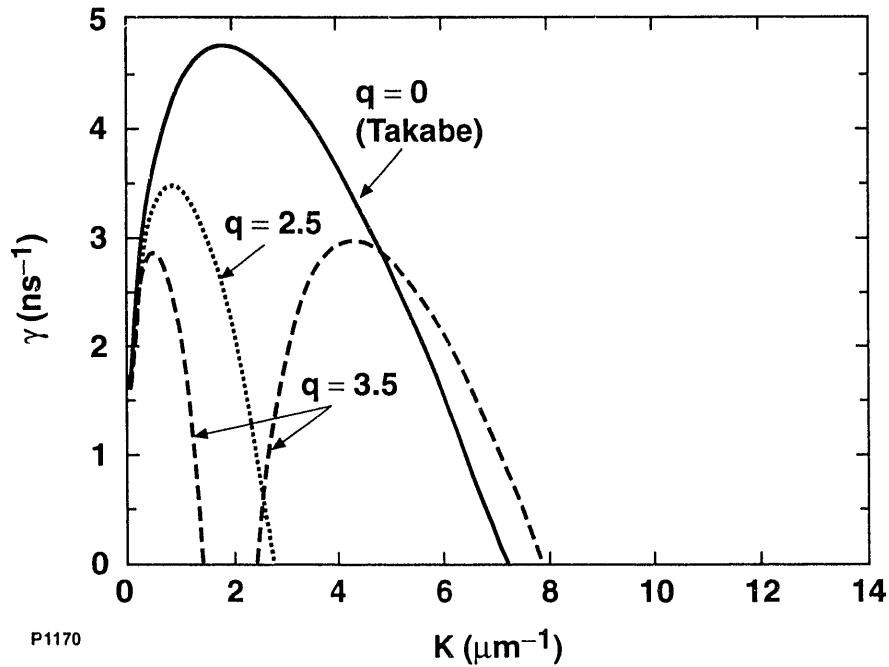
Fig. 2 Plot of the instability growth rate versus the mode wave number k for modulated ( q \neq 0 ) and unmodulated ( q = 0 ) laser intensity.
