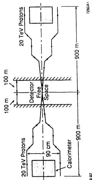
Figure 1. Schematic layout of the FAD collision region.
