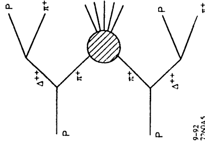
Figure 5. Double-pion exchange mechanism with \Delta^{++} production in the final state.
