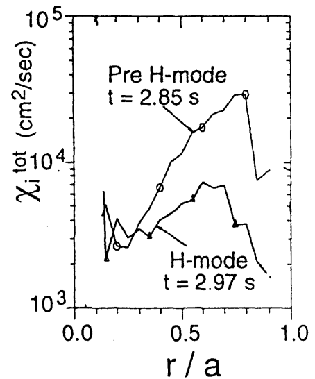
Fig. 2 Total diffusivity, \chi_{i\text{tot}} from TRANSP, as a function of r/a for the DT plasma of Fig. 1; at times before and during H-mode.
