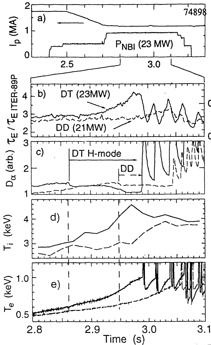
Fig. 1 Time variation of parameters for comparable DD and DT H-modes. Shown are I_p , P_b , \tau_E , D_\alpha , T_i(\text{edge}) , and T_e(\text{edge}) .
