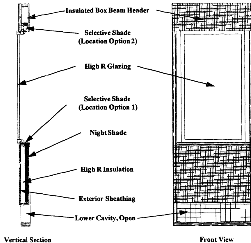
Figure 2 Integrated Window System Components
