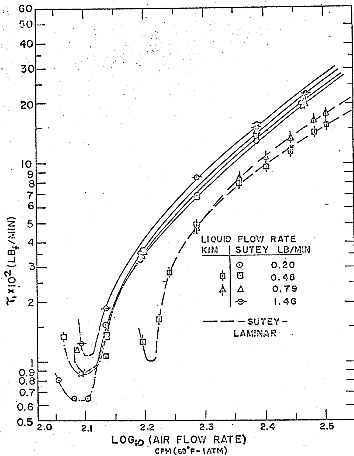
Figure (10) Shear Stress at the Solid-Liquid Film Interface
