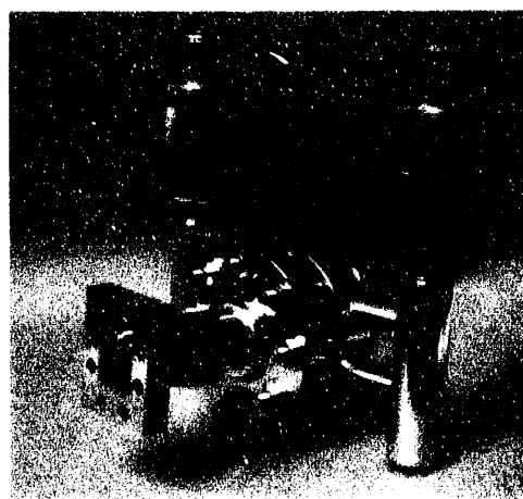
Figure 5. 50 MW Grapefruit Load bakeable to 550°C
