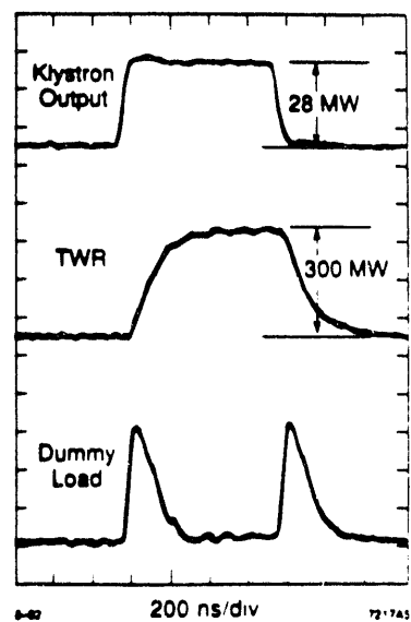
Figure 2. TWR Waveforms
