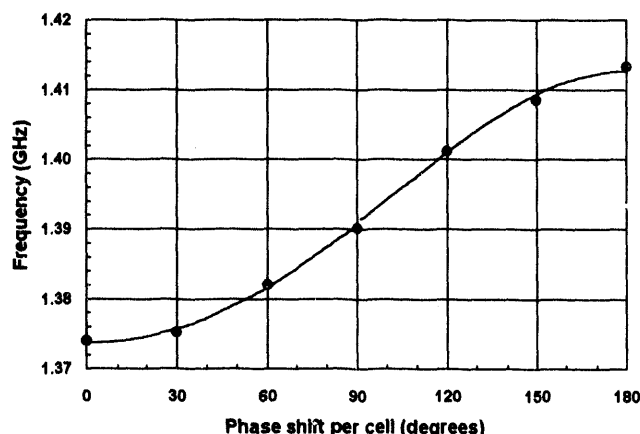
Figure 9. Dispersion curve fitted to the 7-cell CCDTL modes for a single stem. The stopband is +1.1 MHz and the first-neighbor coupling is 2.7\% .
