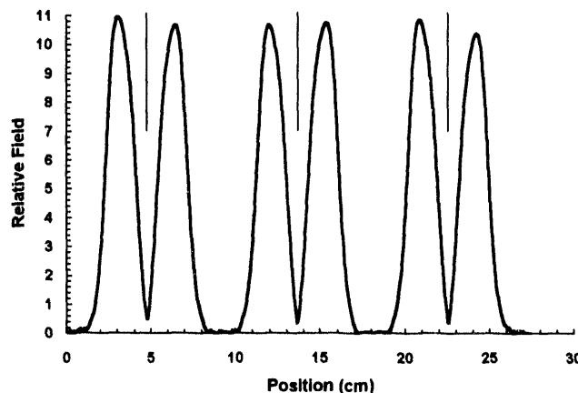
Figure 10. Results of an axial bead-perturbation measurement for the \pi/2 mode of the 7-cell CCDTL model. Vertical lines show the boundaries between accelerating cavities.
