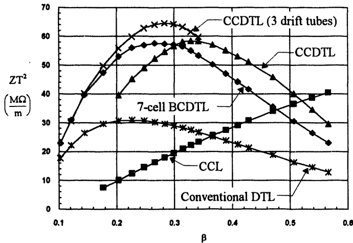
Figure 5. ZT^2 versus particle velocity from Figure 4 corrected for power losses not included by SUPERFISH. Also shown are curves for a CCDTL with 3 drift tubes per cavity and a conventional DTL with drift tubes large enough for focusing magnets.
