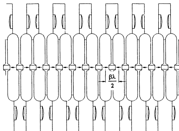
Figure 2. A coupled-cavity linac structure for the same particle velocity as the CCDTL in Fig. 1.
