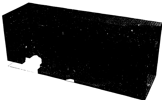
Figure 7. MAFIA-generated mesh and electric field for the 1400-MHz CCDTL operating mode. Though this plot shows only part of the coupling cell, the model included the full geometry of the coupling cells.
