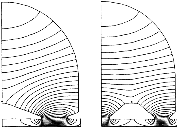
Figure 3. Two CCDTL half cavities. The bottom of each figure is the beam axis and the left-hand edge is a symmetry plane. The contours are SUPERFISH-calculated lines of constant rH . The one-drift-tube cavity at left is for \beta = 0.314 (50-MeV protons). The two-drift-tube cavity at right has the same length and is for \beta = 0.188 (17.1-MeV protons).
