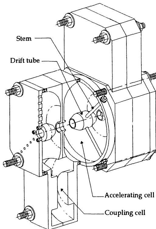
Figure 8. Cut-away view of the CCDTL low-power model. The parts can be assembled with either full or half cells of either accelerating cells or coupling cells on the ends. A separate ring holds the drift tube. This view shows two stems in one of many possible orientations.
