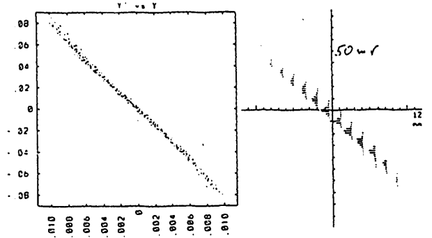
Fig. 3 WARP3D simulation and measured phase-space distributions. Scaled version of a 1MeV,787mA (30keV,4.1mA) beam.
