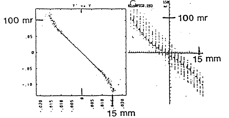
Fig. 2 WARP3D simulation and measured phase-space distributions. Scaled version of a 570keV,787mA (36keV,12.6mA) beam.
