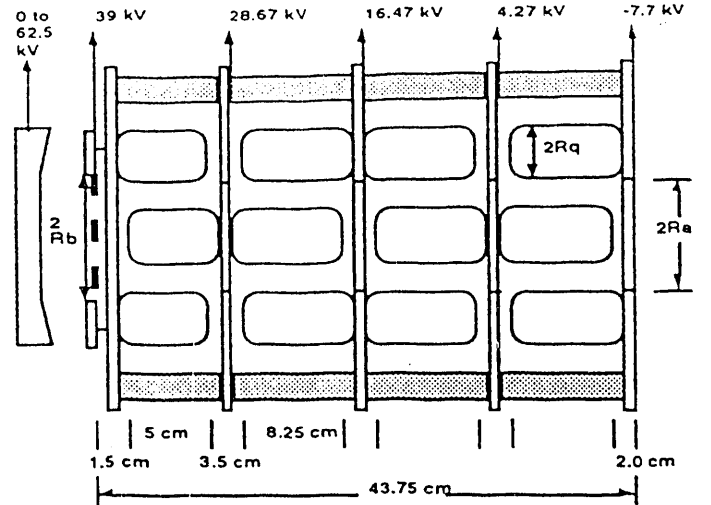
Fig. 1 Schematics of the ESQ-Scaled Experiment. Cross-sectional view.
