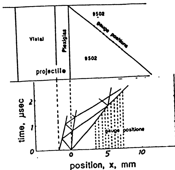
Figure 1. Experimental arrangement and x-t diagram showing preshock and main shock generation for a PBX-9502 experiment.
