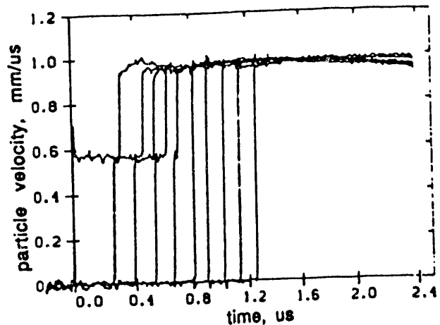
Figure 2. Data from experiment on PBX-9502 with P_1 = 3.71 GPa, t_1 = 0.32 \mu s, and P_2 = 8.19 GPa.
