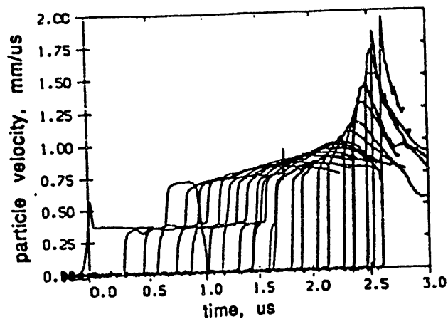
Figure 3. Data from two experiments on PBX-9404, showing growth of reactive wave in preshocked material: P_1 = 2.3 GPa, t_1 = 0.68 \mu s, P_2 = 5.6 GPa.
