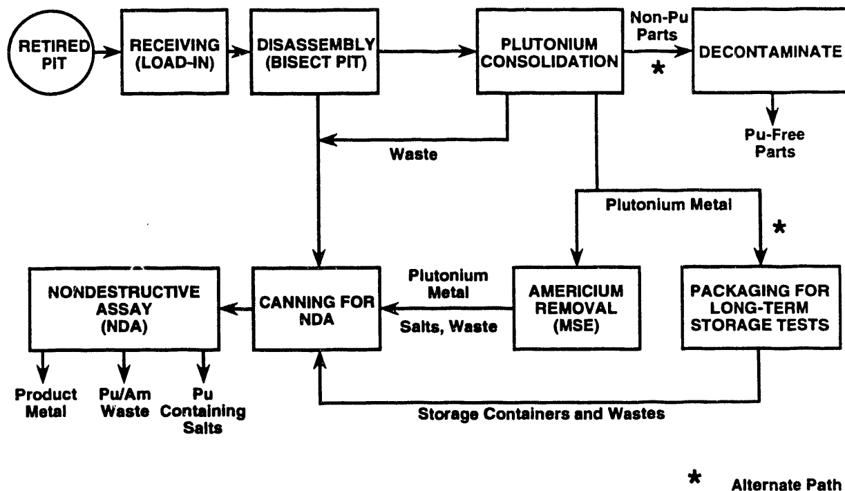
Fig. 1. Materials flow in the ARIES process.
