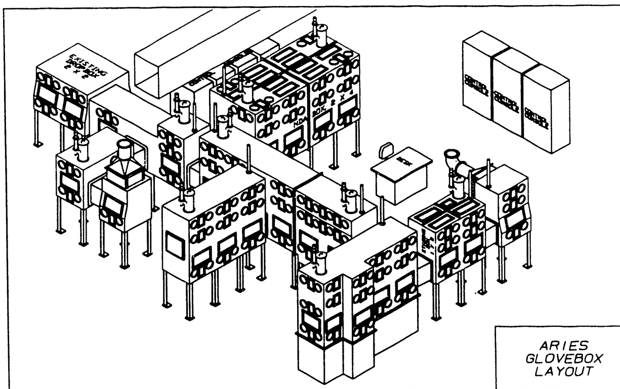
Fig. 2. The ARIES glove-box line.
