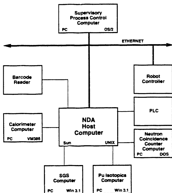
Fig. 3. The ARIES NDA subsystem.
