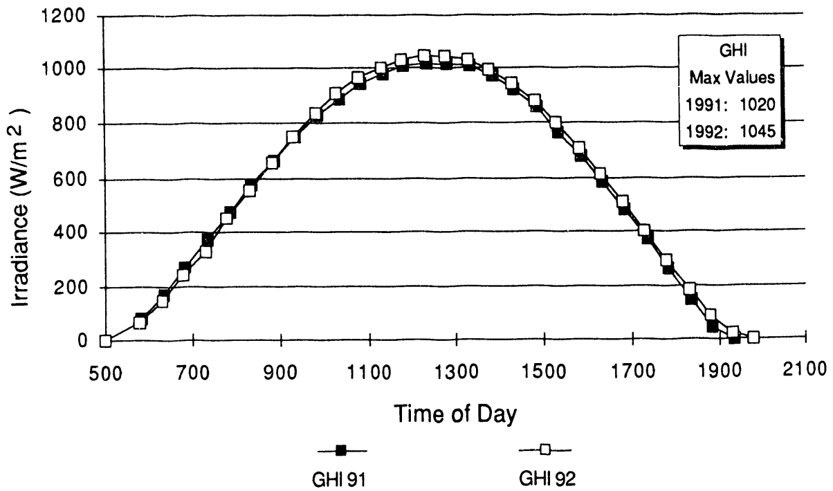
Figure 5-7. Global Horizontal Irradiance -- Albuquerque, New Mexico 6/16/91, 6/14/92.
