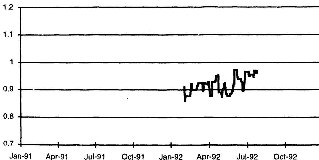
Figure 5-3. Clear Sky DNI Quotients -- Albuquerque, NM 1992/1991.
