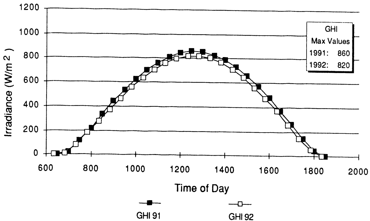
Figure 5-5. Global Horizontal Irradiance -- Albuquerque, New Mexico 3/8/91, 3/6/92.
