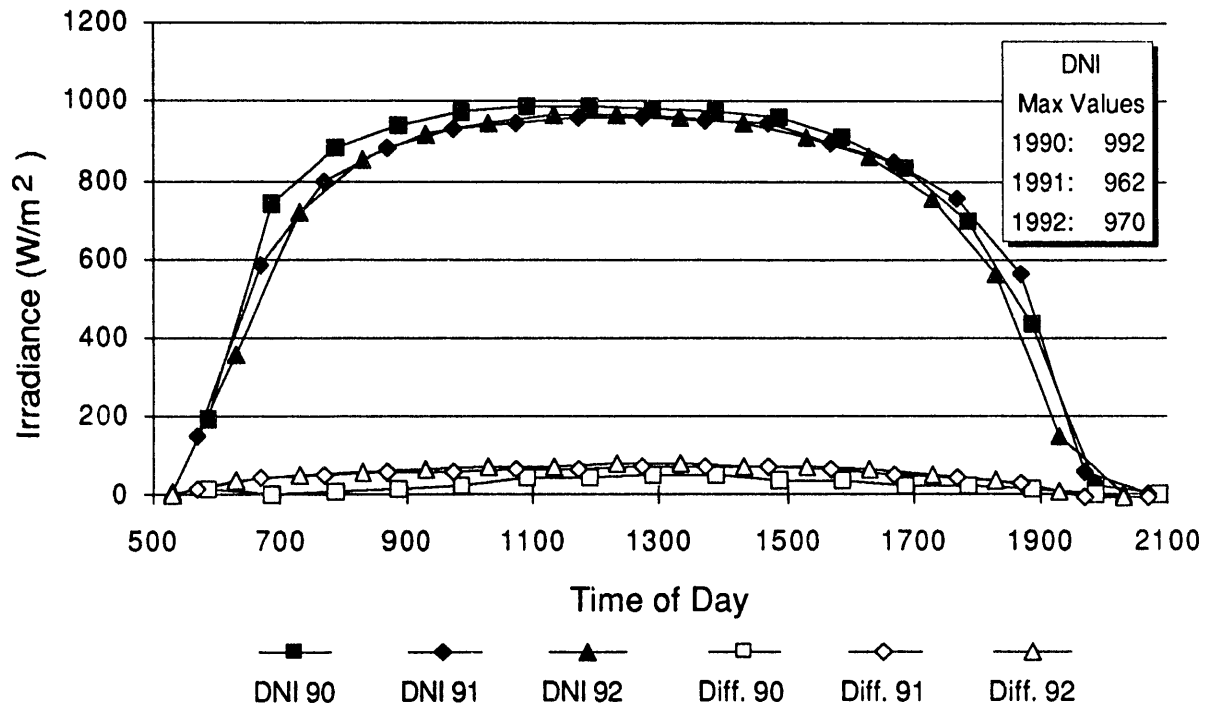
Figure 2-6. Direct Normal and Diffuse Irradiance -- Las Cruces, New Mexico 7/17/90, 7/17/91, 7/16/92.
