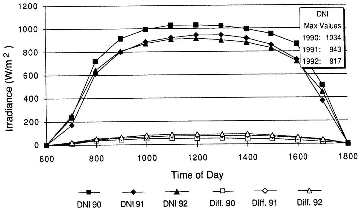
Figure 3-6. Direct Normal and Diffuse Irradiance -- Golden, Colorado 10/21/90, 10/21/91, 10/10/92.
