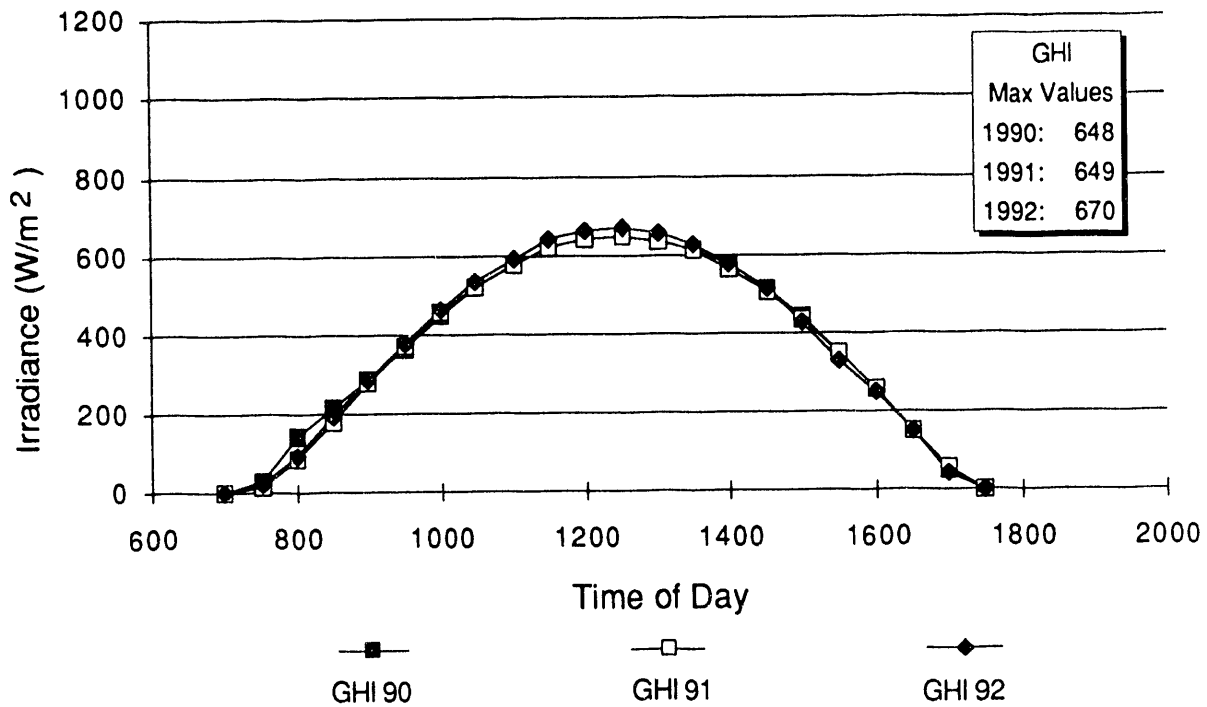
Figure 4-5. Global Horizontal Irradiance -- Carrisa Plains, California 1/21/90, 1/23/91, 1/23/92.
