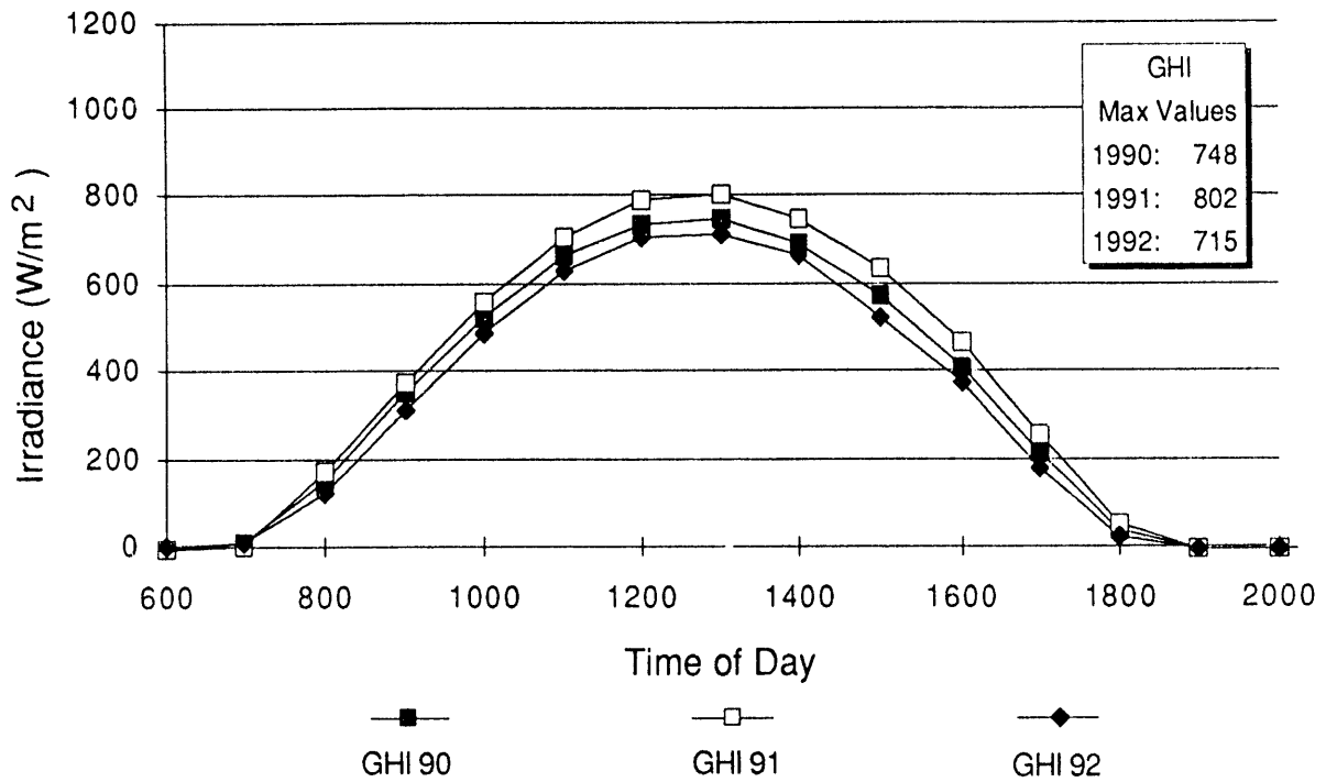
Figure 3-5. Global Horizontal Irradiance -- Golden, Colorado 3/2/90, 3/7/91, 2/28/92.
