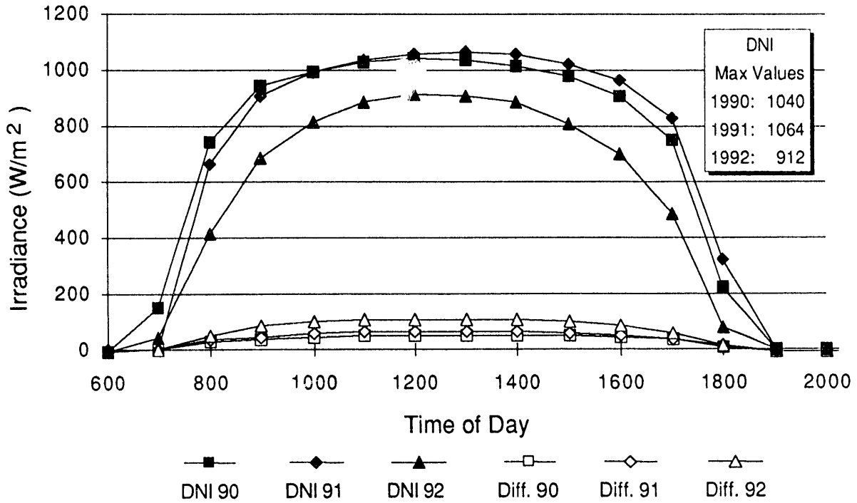
Figure 3-4. Direct Normal and Diffuse Irradiance -- Golden, Colorado 3/2/90, 3/7/91, 2/28/92.
