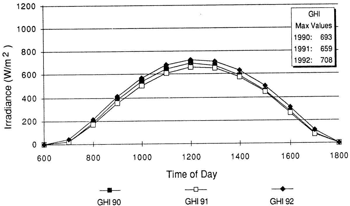
Figure 3-7. Global Horizontal Irradiance -- Golden, Colorado 10/21/90, 10/21/91, 10/10/92.
