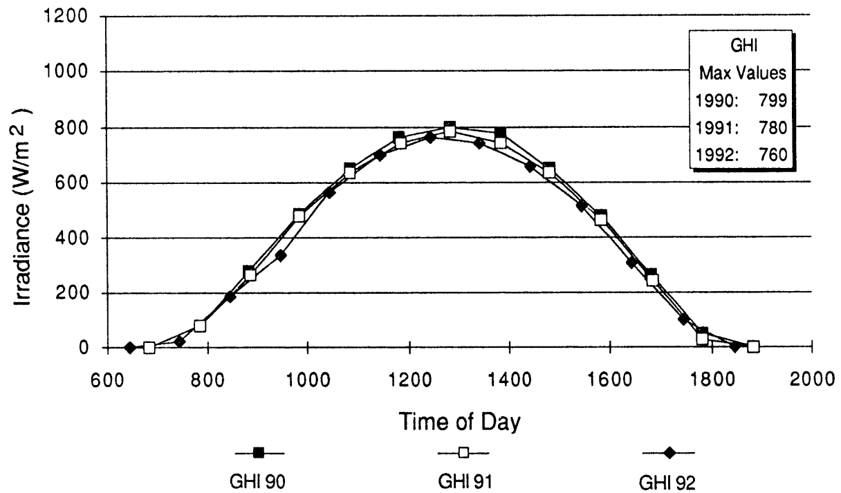
Figure 2-5. Global Horizontal Irradiance -- Las Cruces, New Mexico 2/16/90, 2/14/91, 2/14/92.
