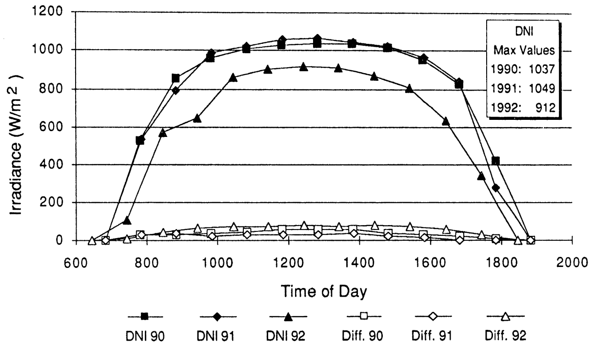
Figure 2-4. Direct Normal and Diffuse Irradiance -- Las Cruces, New Mexico 2/16/90, 2/14/91, 2/14/92.
