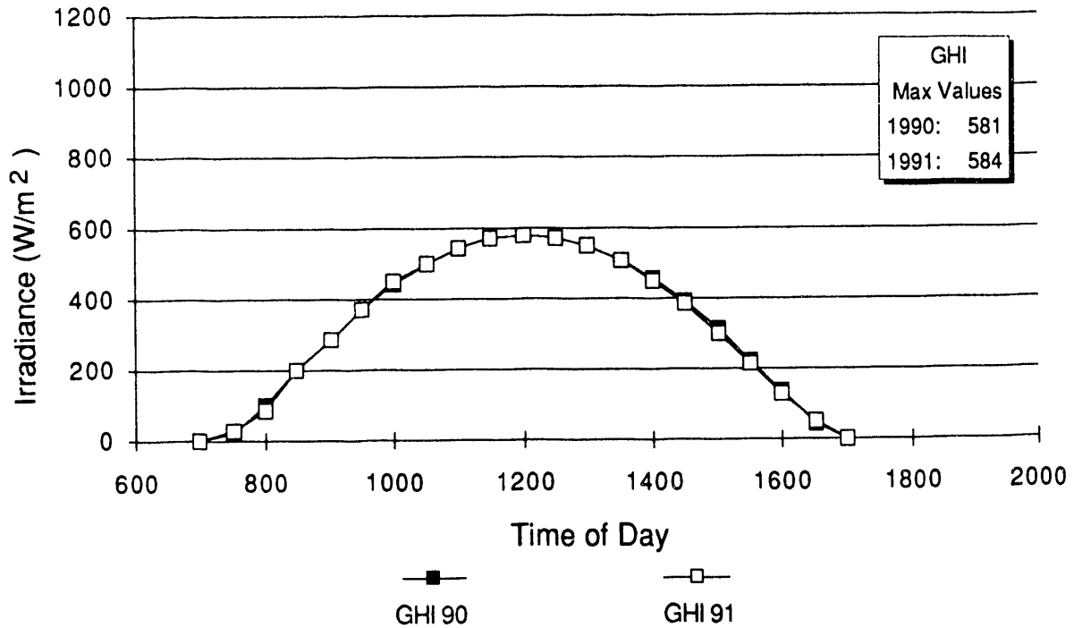
Figure 4-7. Global Horizontal Irradiance -- Carrisa Plains, California 12/8/90, 12/4/91.
