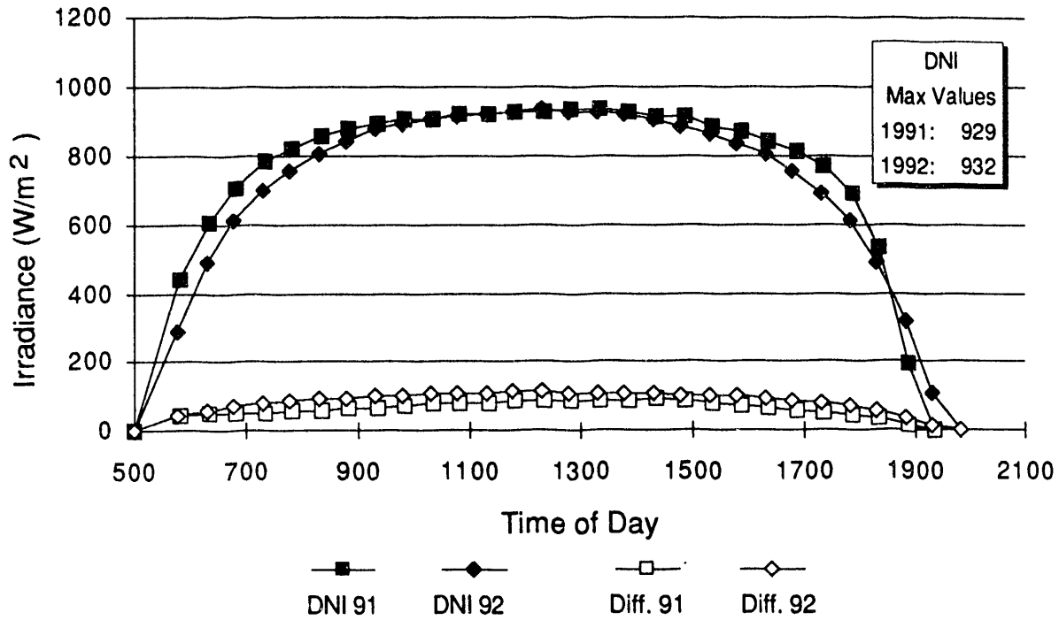
Figure 5-6. Direct Normal and Diffuse Irradiance -- Albuquerque, New Mexico 6/16/91, 6/14/92.
