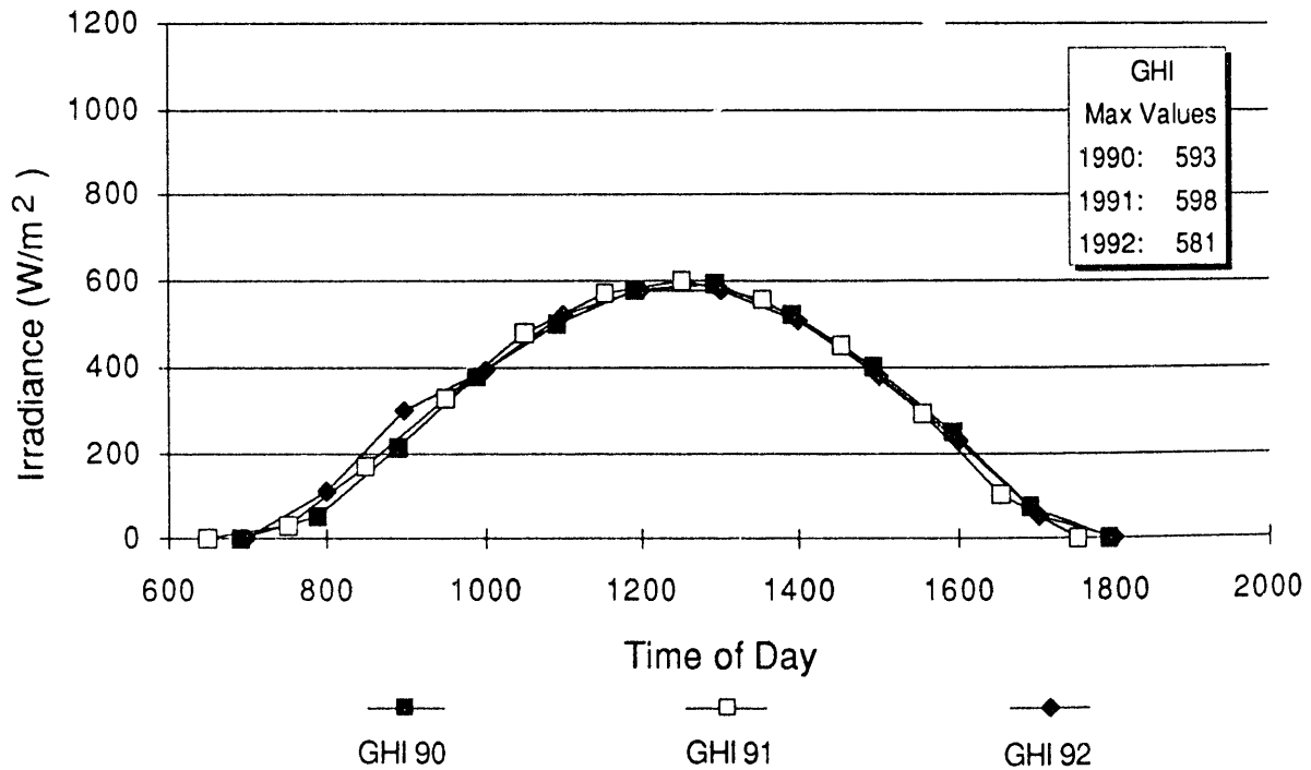
Figure 2-9. Global Horizontal Irradiance -- Las Cruces, New Mexico 12/11/90, 12/12/91, 12/9/92.
