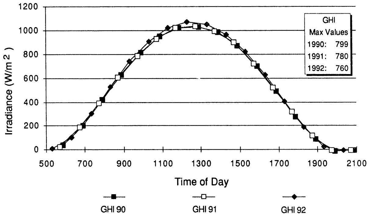
Figure 2-7. Global Horizontal Irradiance -- Las Cruces, New Mexico 7/17/90, 7/17/91, 7/16/92.
