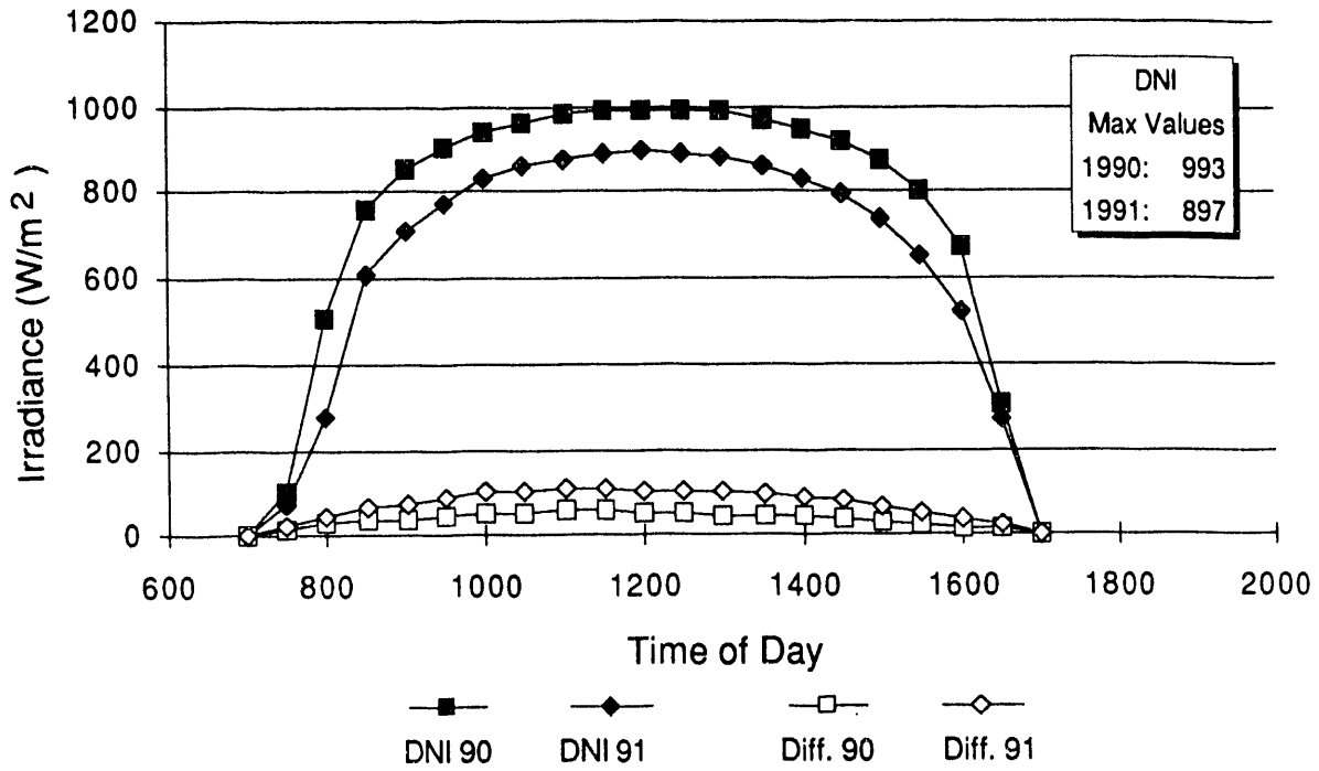
Figure 4-6. Direct Normal and Diffuse Irradiance -- Carrisa Plains, California 12/8/90, 12/4/91.
