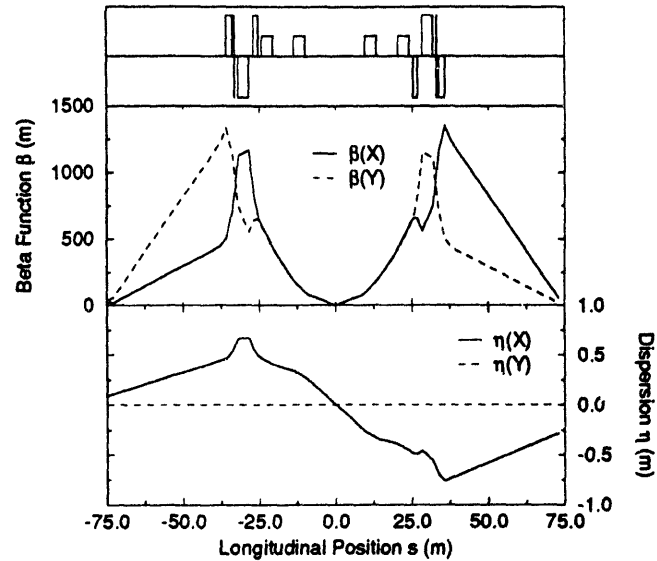
Figure 1: Optical functions near the 8 o'clock IR and the PHENIX experimental area for a \beta^* = 1 m lattice. Longitudinal position is measured from the interaction point. The positions of IR quads 1-3, IR skew quad correctors (next to IR quad 3), and the DX and D0 dipoles are also shown.
