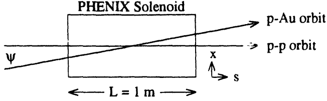
Figure 2: Orbit through the PHENIX solenoid, for proton-proton and proton-gold collisions. The orbit skew angle is \psi = 3.85 mrad.
