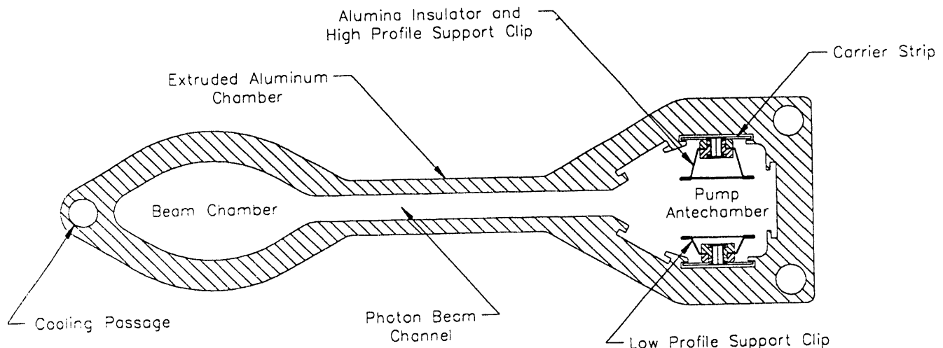
Figure 1. Storage Ring Vacuum Chamber Cross Section.
