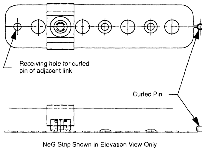
Figure 4. Typical Link.
