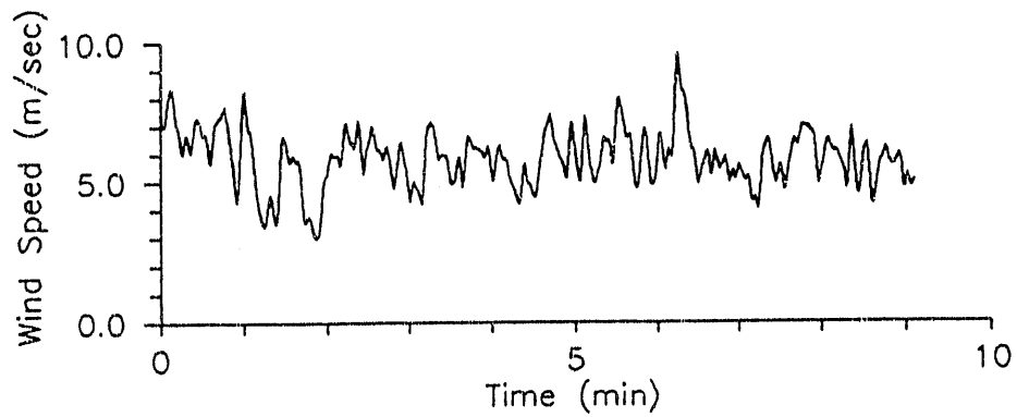
Figure 2c. Wind Speed SHG Time Series, 6/10/88
