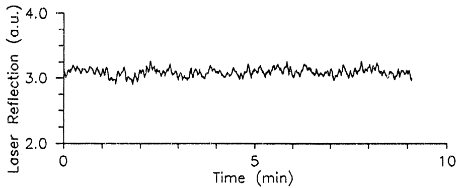
Figure 2b. 532-nm Laser Reflection Time Series, 6/10/88
