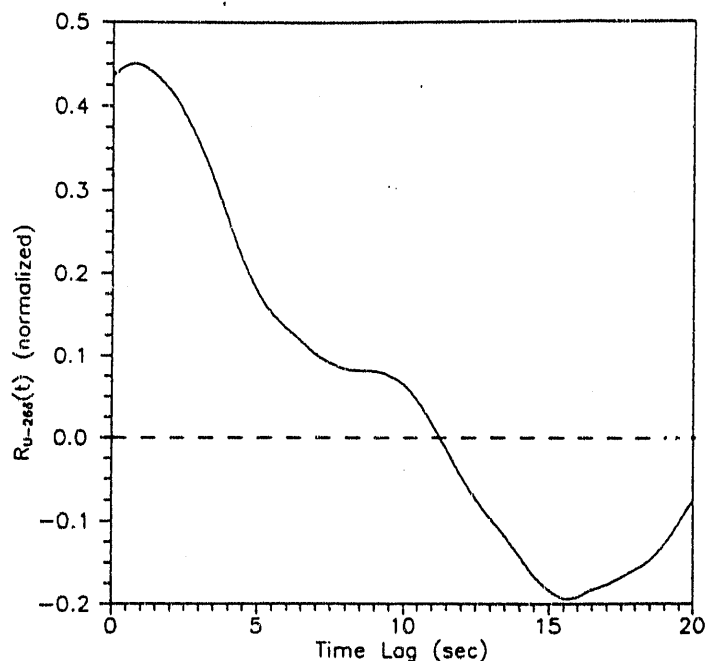
Figure 3a. U-266 Cross-Correlation
