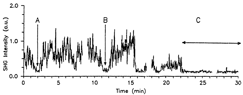
Figure 4. SHG Time Series from Natural Slicks, 10/1/88
