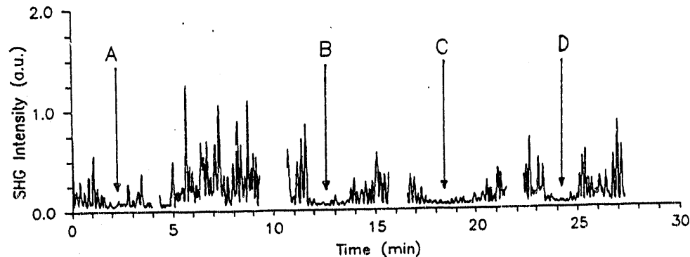
Figure 5. SHG Time Series from Artificial Slicks, 10/9/88
