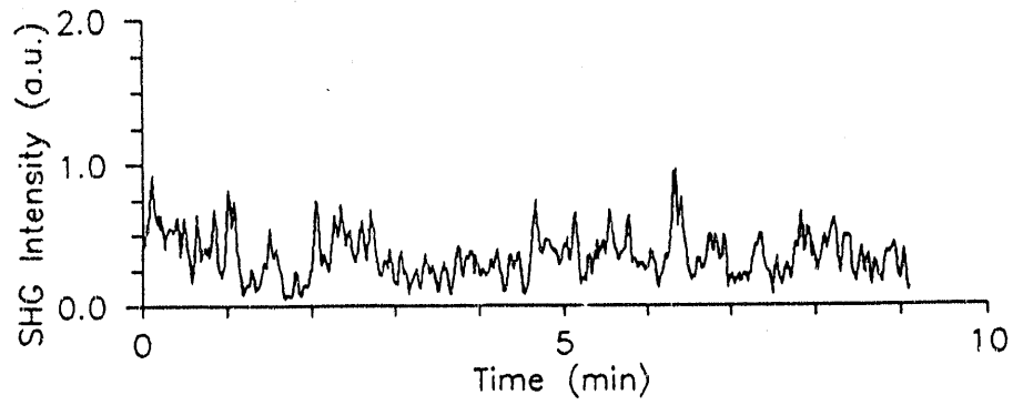
Figure 2a. 266-nm SHG Time Series, 6/10/88
