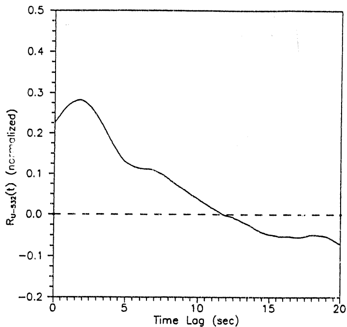
Figure 3b. U-532 Cross-Correlation
