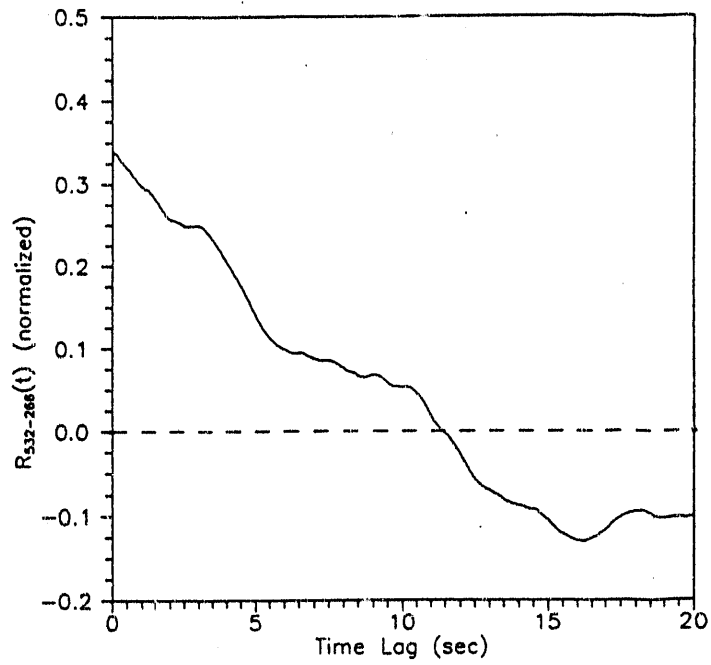
Figure 3c. 532-266 Cross-Correlation
