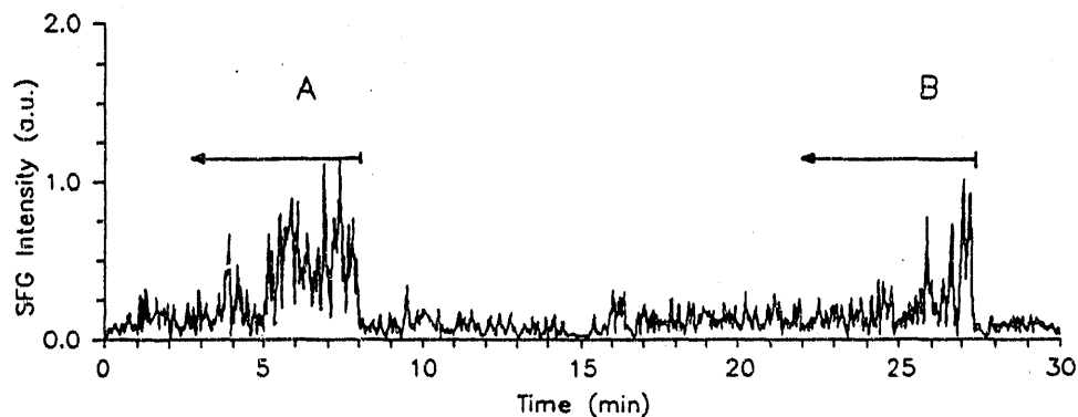
Figure 6. SFG Time Series from Natural Slicks, 10/18/89
