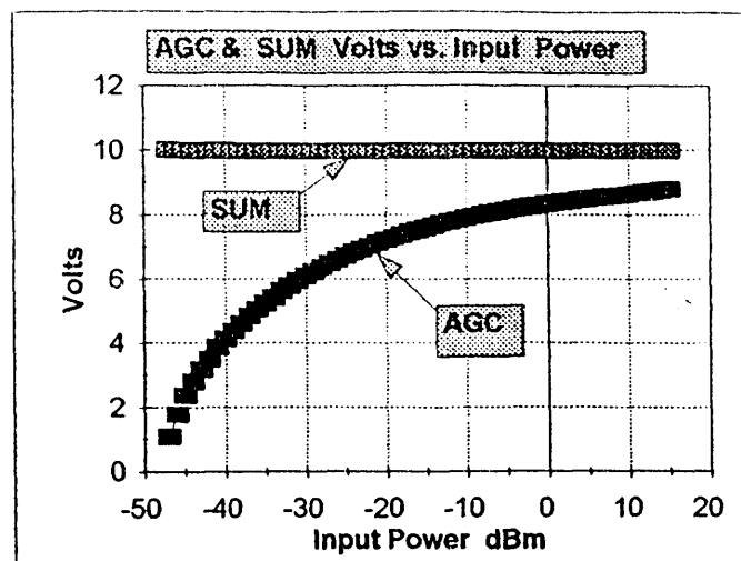
Figure 6. AGC and SUM variation vs. input power.
