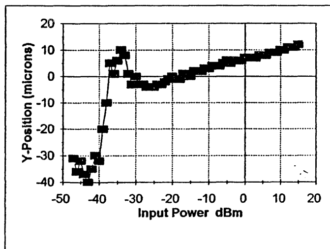
Figure 5. Y - Position variation (3,3 mm) vs. input power.
