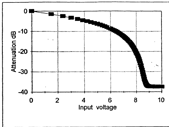
Figure 4. AGC box characteristics.
