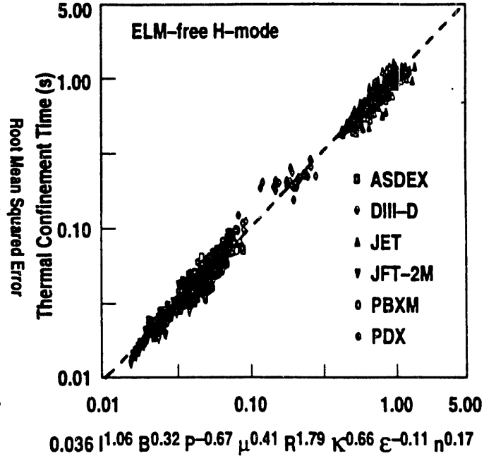
Fig. 2. Observed \tau_{th} versus that predicted from Eq. (1) for the ELM-free standard dataset.
