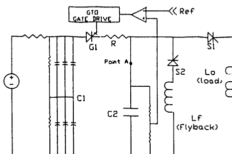
Fig. III.2 System Implementation
