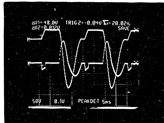
Fig IV.1 Discharge Voltage and Current Measured at Point A in Fig. III.2 (Upper Trace 50V/div) (Lower Trace 100A/div) (Time Base 5ms/div)
