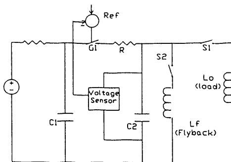
Fig. III.1 Design Configuration
