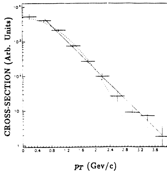
Figure 3: p_t dependence of D^+ production from 250 GeV/c \pi^- . The dashed line is a fit to e^{-bp_t^2} . The solid line, a fit to e^{-b'p_t} , is in better agreement with the data at large p_t .
