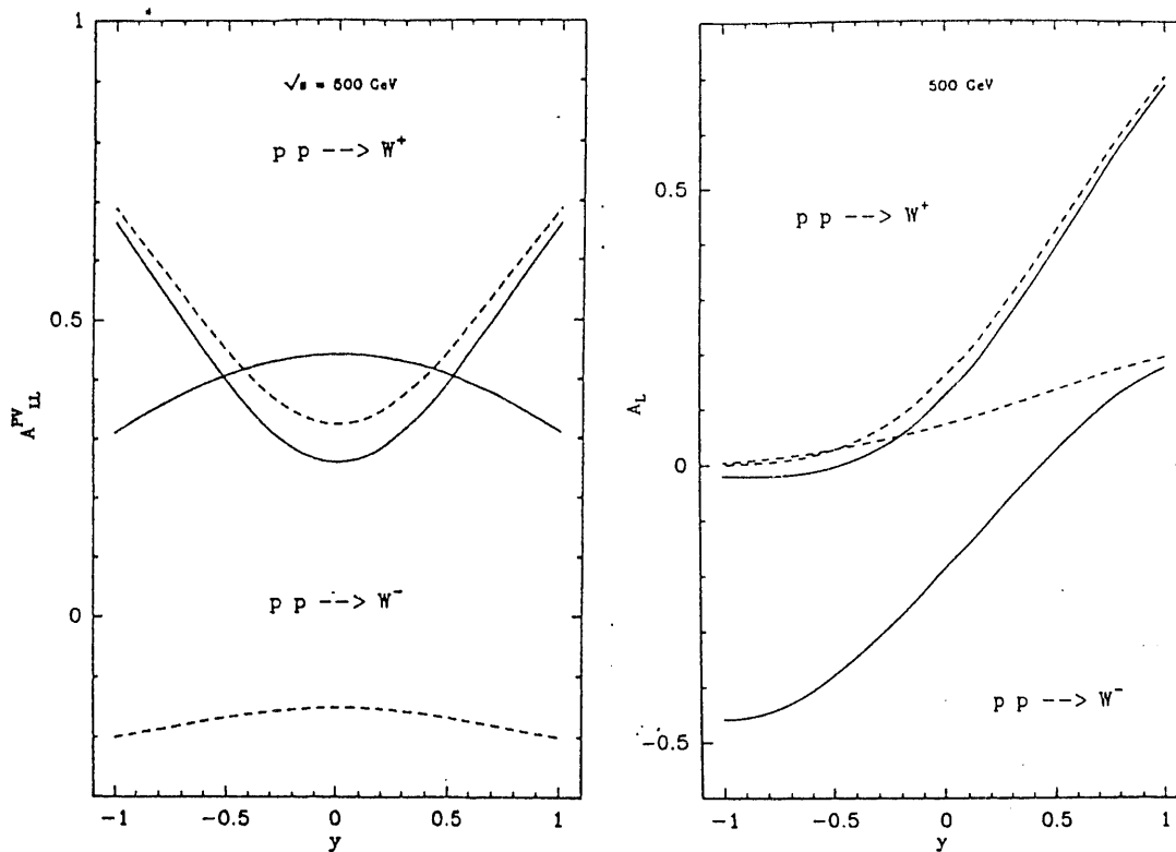
Figure 3. Predictions for Parity violating asymmetries in W production. The solid lines with sea quark polarization, and the dashed lines with zero polarization.
