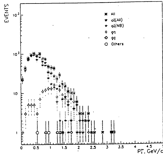
Figure 1. Contributions to the dilepton rates from various partonic processes PHENIX ( \mu\mu ), \sqrt{S}=200 \text{ GeV} , and M_{\mu\mu}=2-3 \text{ GeV}/c^2 .
