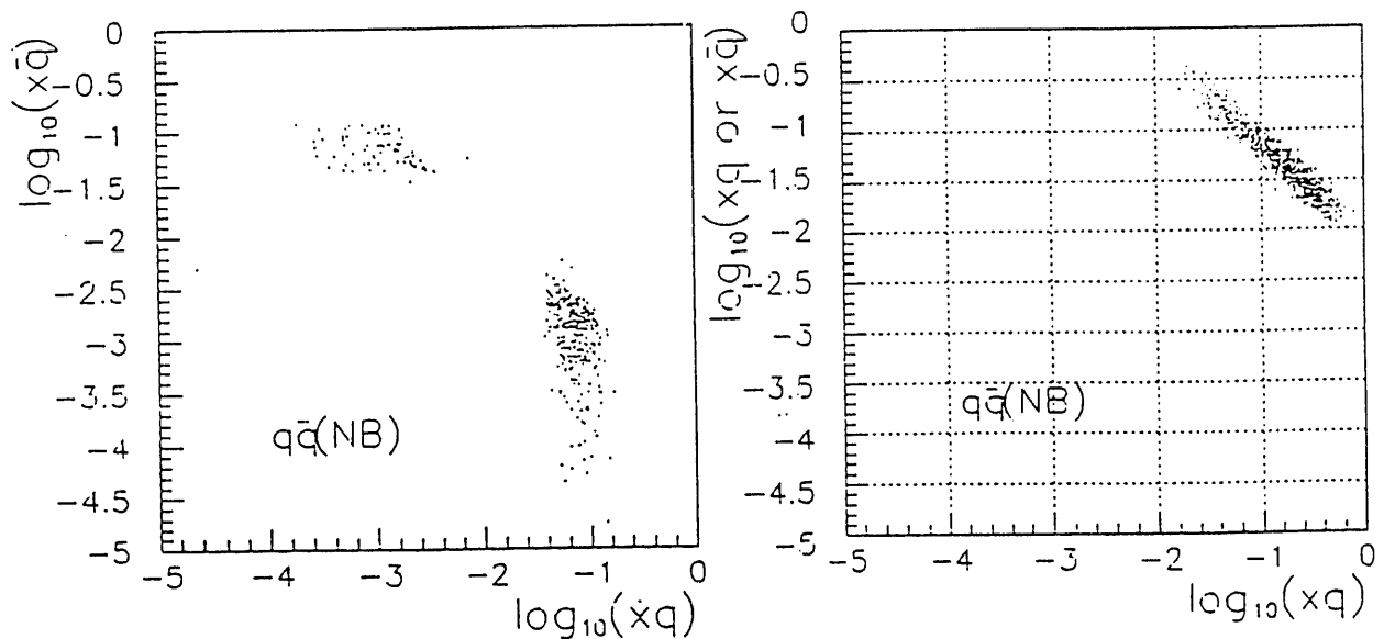
Figure 2. Diplots of the kinematic regions covered by the PHENIX and STAR detectors respectively. The axes refer to the momentum fractions carried by the interacting partons.
