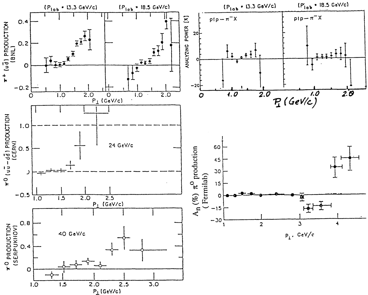
Figure 4. The single spin asymmetry in inclusive pion production versus transverse momentum.
