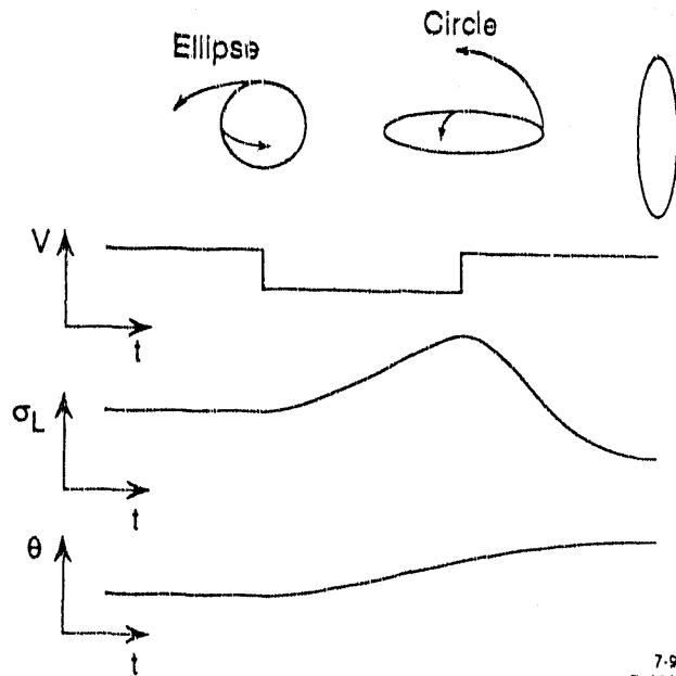
Figure 1: Principle of pre-compression in the DR.
