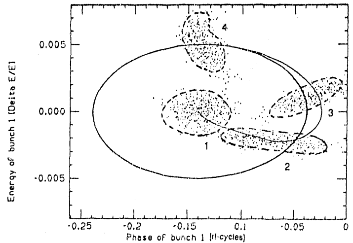
Figure 2: Pre-compression simulation.
