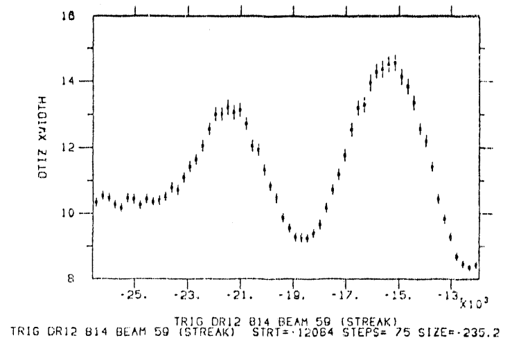
Figure 4: Bunch length measurement by a streak camera.
