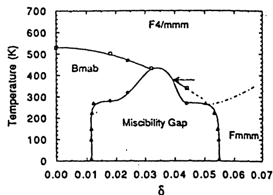
Figure 1. Phase diagram of \text{La}_2\text{CuO}_{4+\delta} [4].
