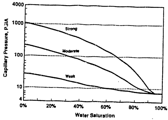
Figure 6 Matrix Capillary Pressure
