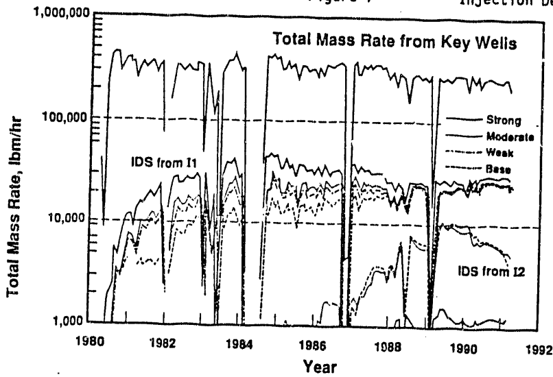
Figure 8 Key Wells Modeled Injection Derived Steam
