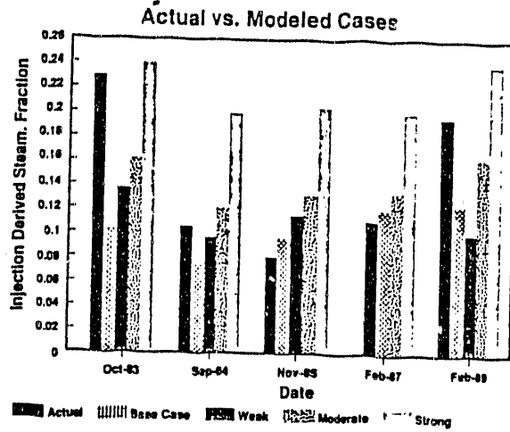
Figure 7 Injection Derived Steam Results for Well P5
