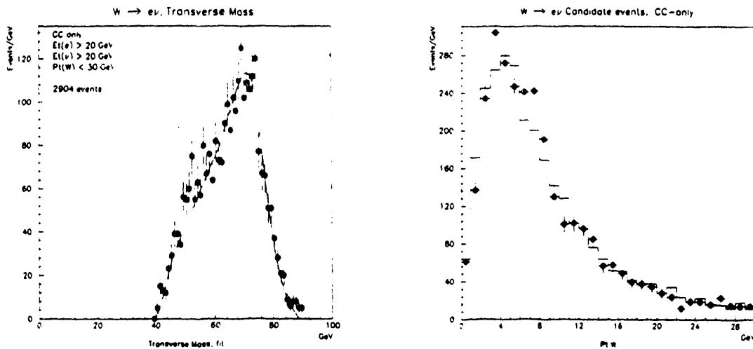
Figure 3: Distribution of the transverse mass (a) and the W transverse momentum of W^\pm \rightarrow e^\pm \nu_e events. The points are the data; the solid line is the fit.
